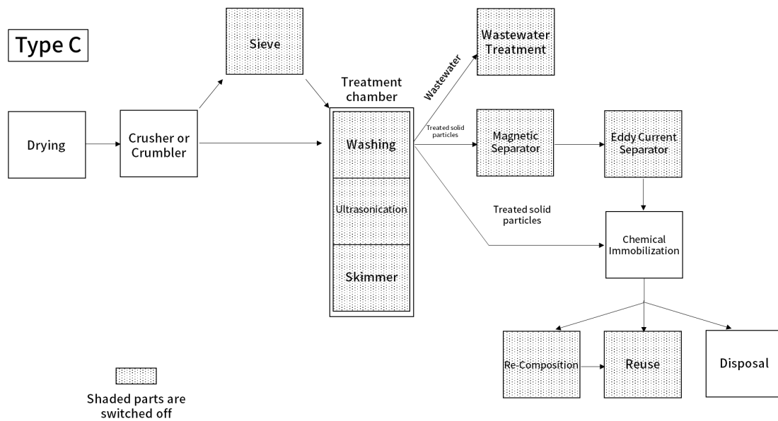
Figure 4: Type C solid waste treatment scheme
