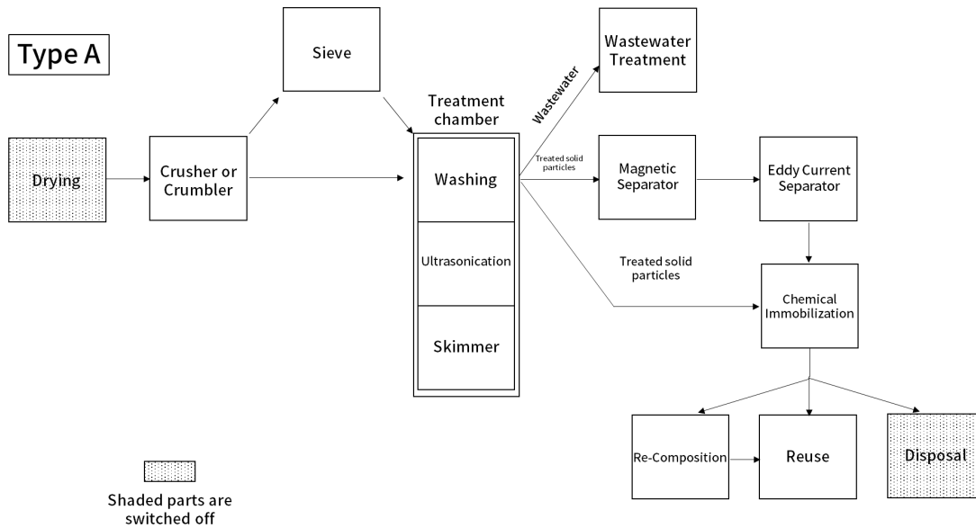
Figure 2: Type A solid waste treatment scheme
