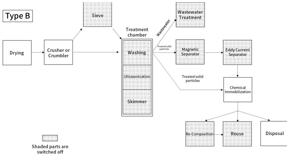
Figure 3: Type B solid waste treatment scheme
