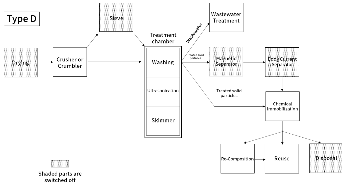
Figure 5: Type D solid waste treatment scheme
