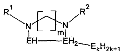
(R^1N(CH_2)_mNR^2)EHEH_2E_kH_{2k+1} Compound B
