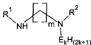
R^1NH(CH_2)_mNR^2E_kH_{(2k+1)} Compound A
