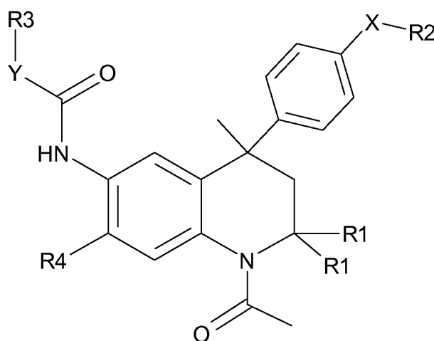
Formula I
