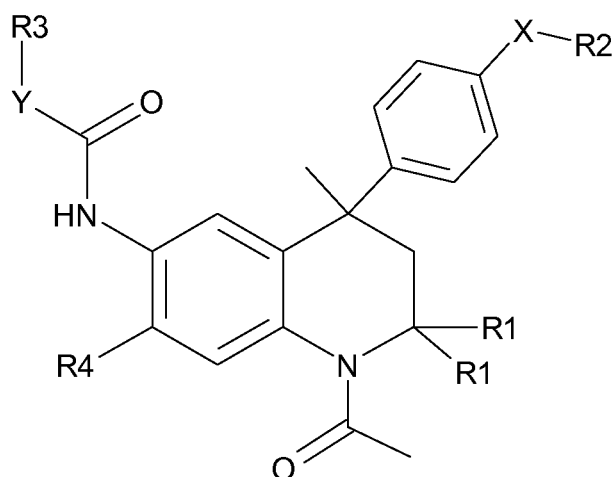
Formula I
