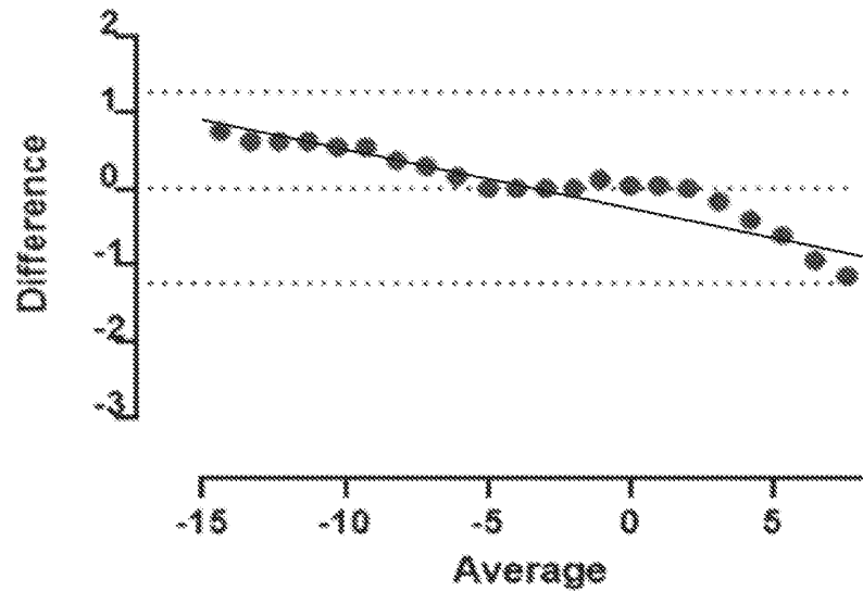
Difference vs. average: Bland-Altman of Model Eye K900 Aurorefractor
