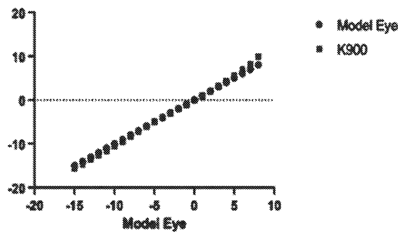
XY data: Correlation of Model Eye K900 Autorefractor (full)
