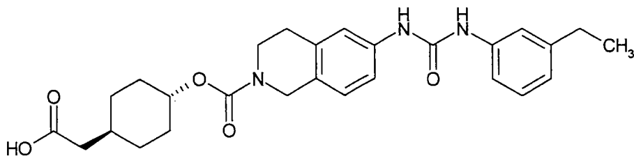
(70a) 6-[3-(3-ethyl-phenyl)-ureido]-3,4-dihydro-1H-isoquinoline-2-carboxylic acid tert-butyl ester
