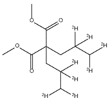
Dimethyl 2,2-bis(2,2,3,3-tetradeuteriopropyl)propanedioate
