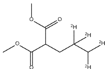
Dimethyl 2-(2,2,3,3-tetradeuteriopropyl)propanedioate
