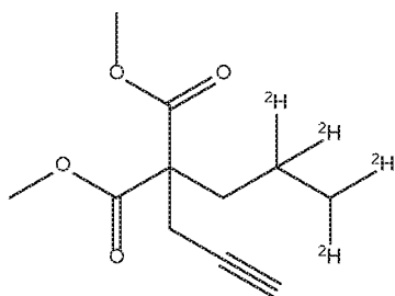
Dimethyl 2-prop-2-ynyl-2-(2,2,3,3-tetradeuteriopropyl)propanedioate
