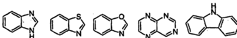
Benzimidazole Benzthiazole Benzoxazole Pteridine Carbazole
