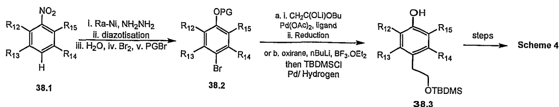
Scheme 11.2
