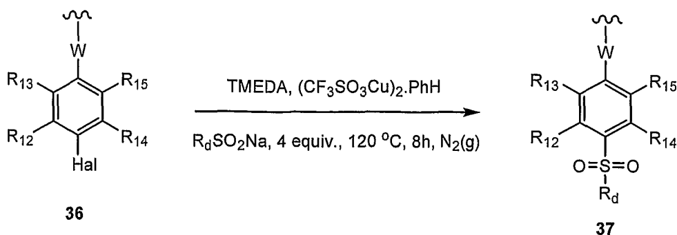
Scheme 10
