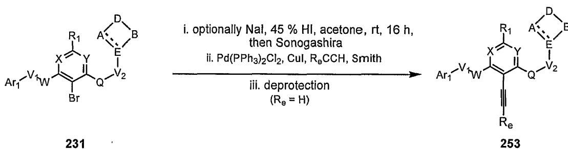
Scheme 5.3
