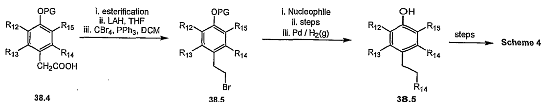
Scheme 11.2
