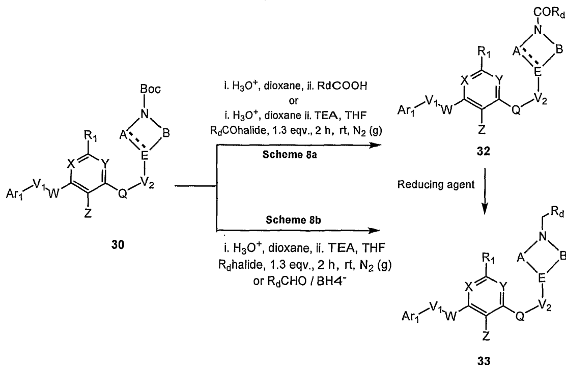
Scheme 8
