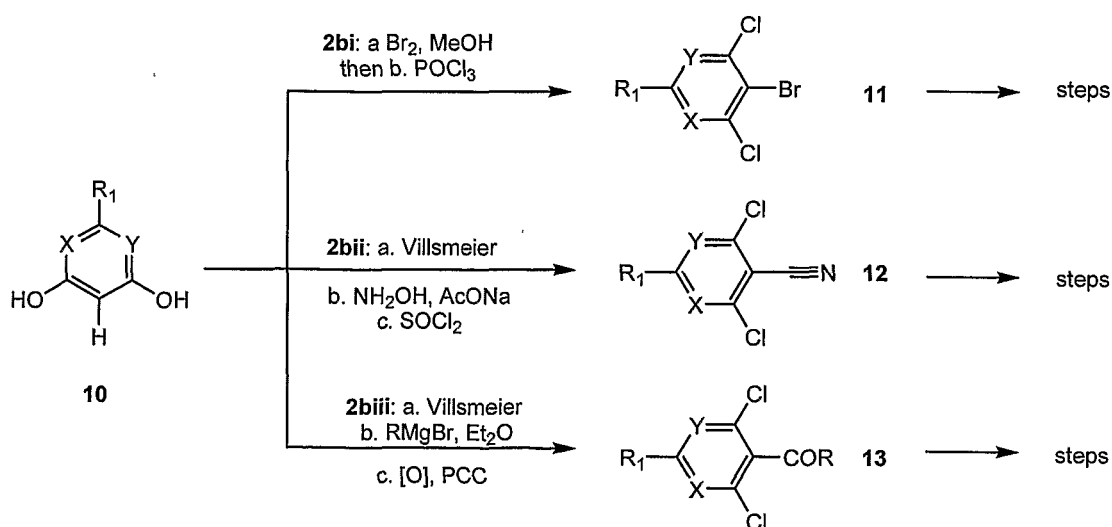
Scheme 2b
