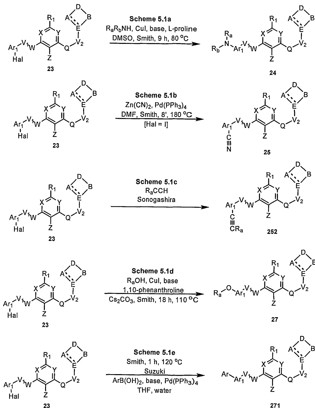
Scheme 5.1
