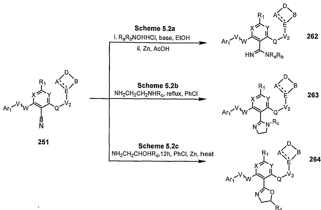
Scheme 5.2
