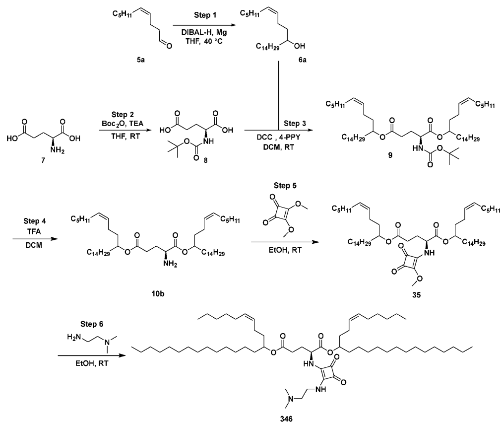
[01065] Scheme 11
