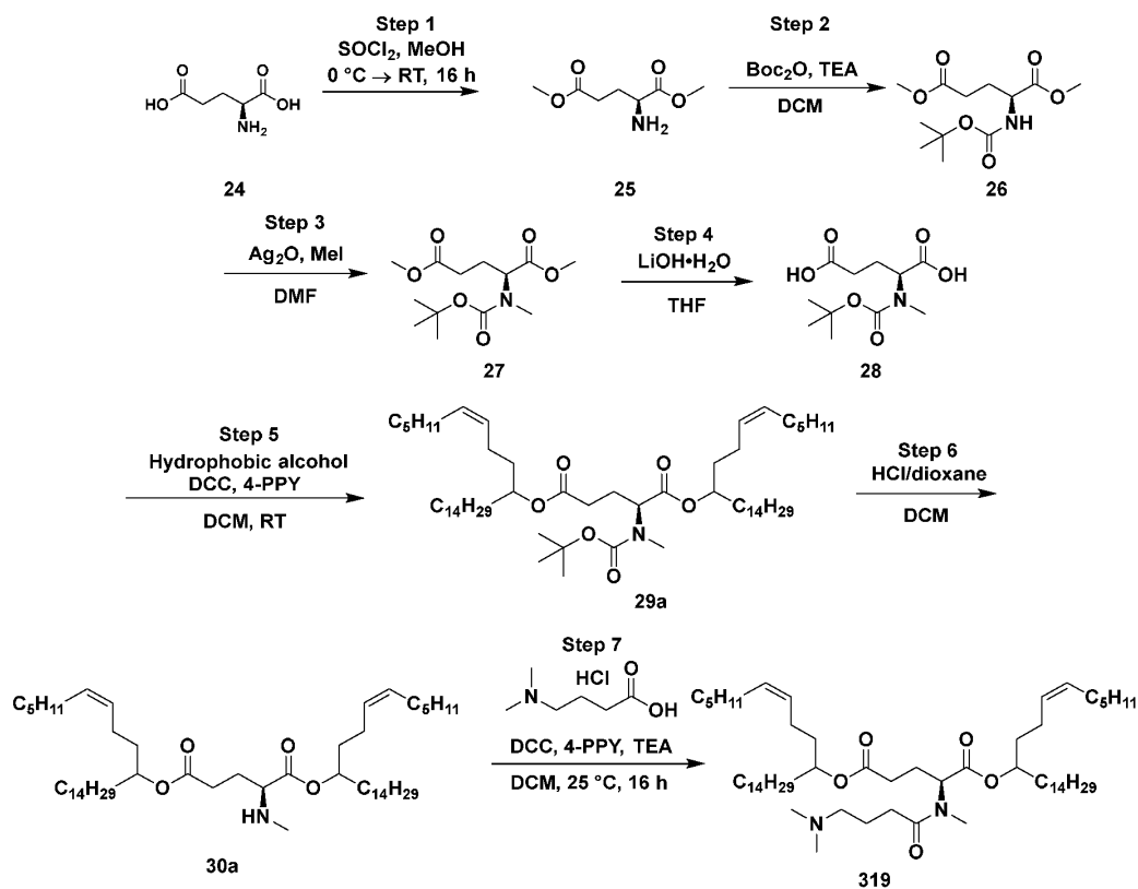
[01075] Scheme 12
