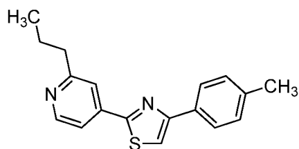
Fatostatin
