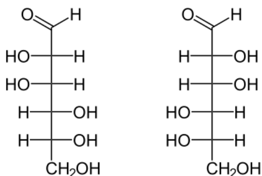
D-Mannose
