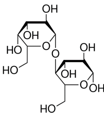
beta-lactose,
