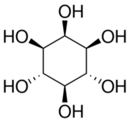
Inositol, and
