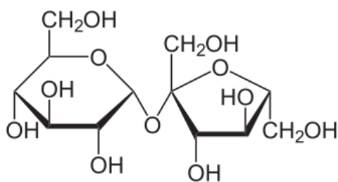
Sucrose,
