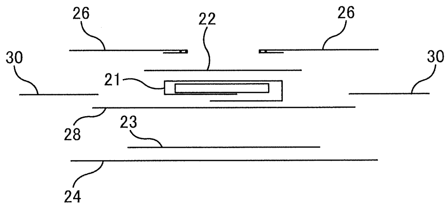
FIG. 2C (REAR PORTION 7)
