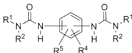
Formel (VI)
