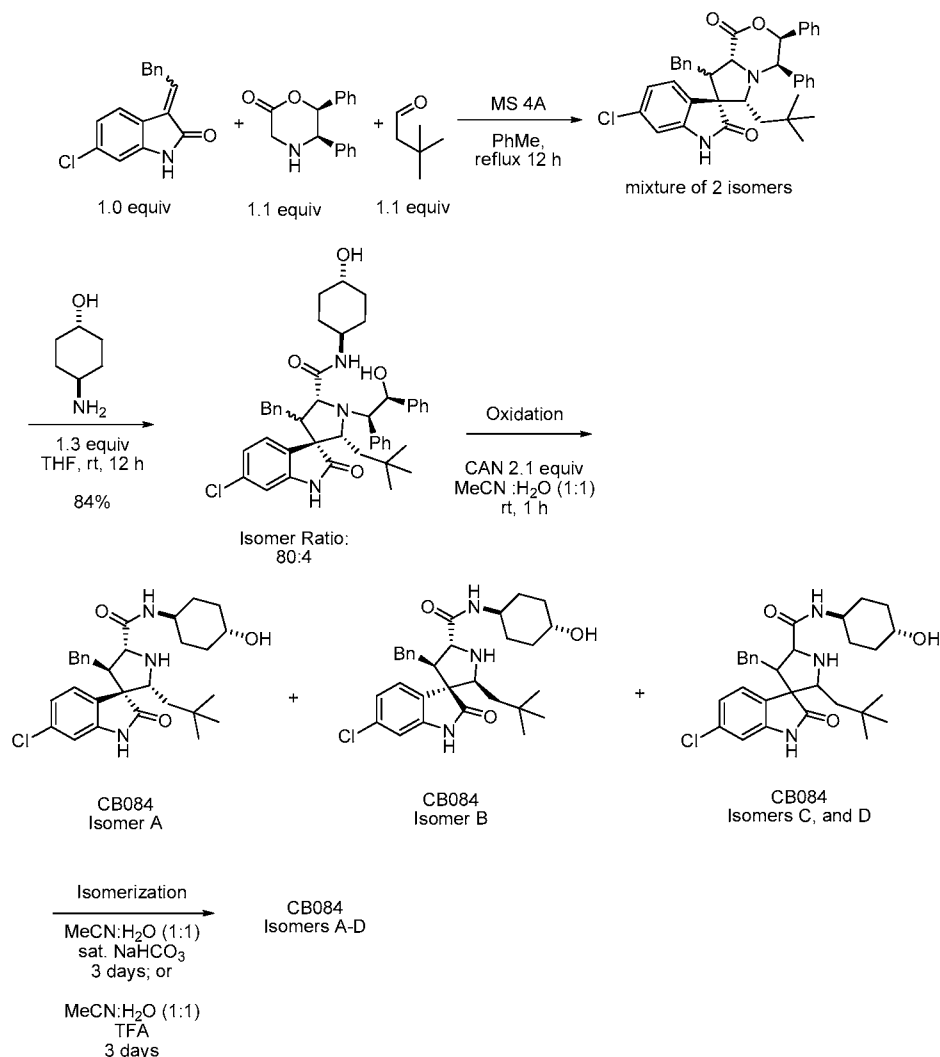
Scheme 15
