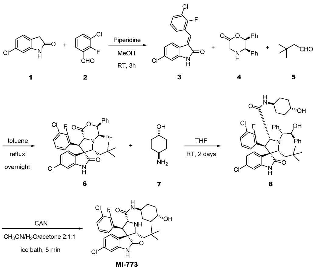
Scheme 8
