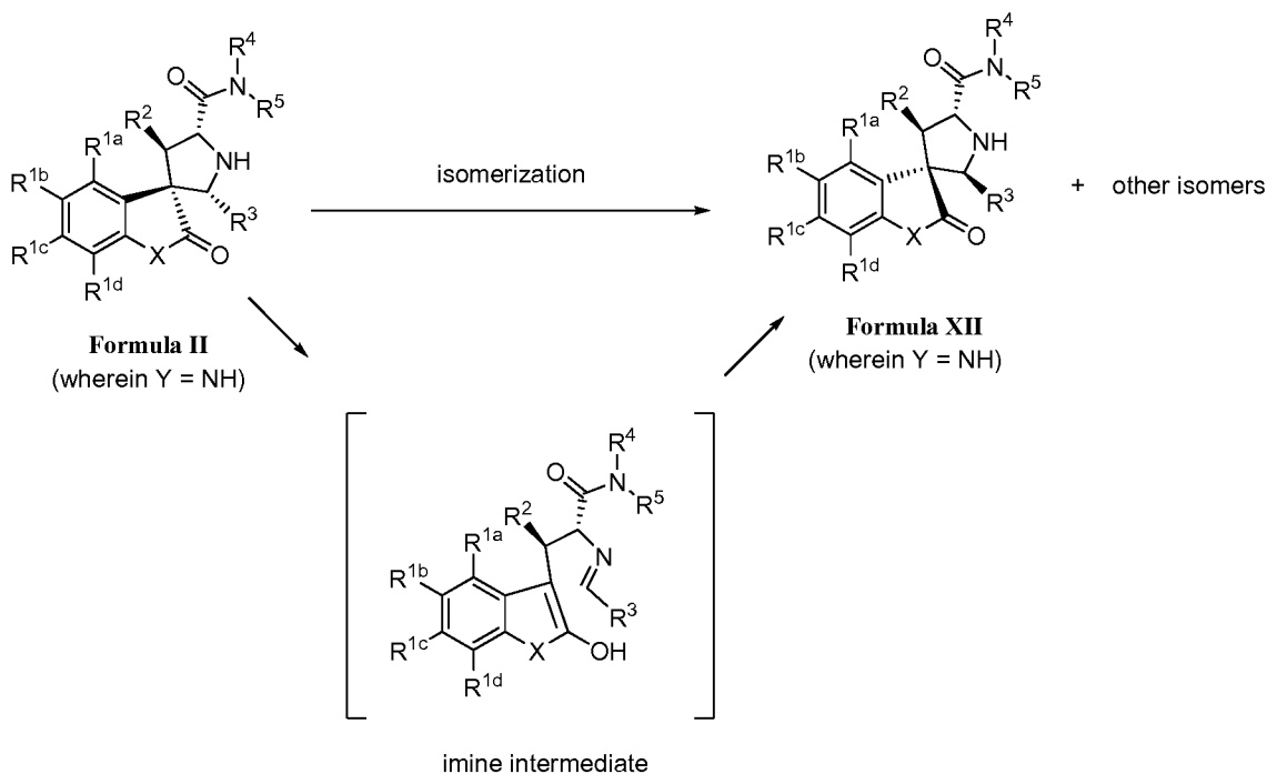
Scheme 5
