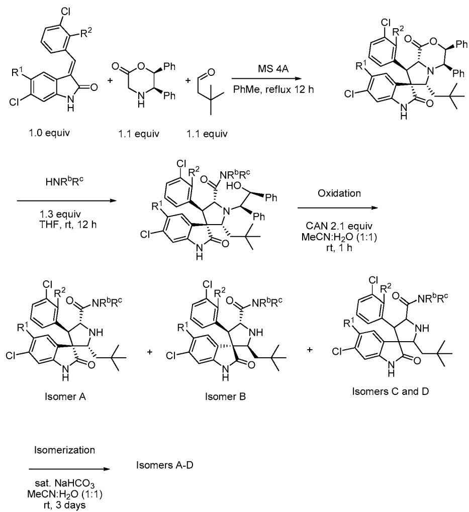
Scheme 10
