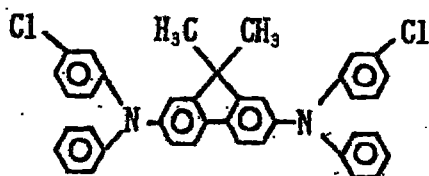
Exemplary Compound (4)-57
