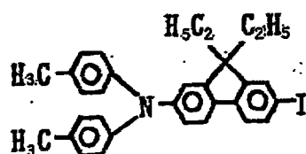
Exemplary Compound (4)-60
