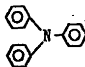
Exemplary Compound (4)-26
