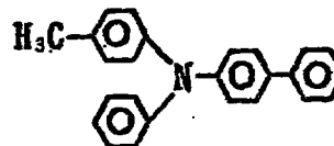
Exemplary Compound (4)-8
