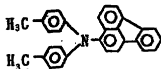
Exemplary Compound (4)-34
