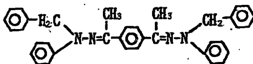
Exemplary Compound (5)-30
