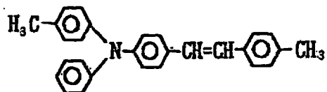
Exemplary Compound (3)-21
