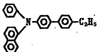
Exemplary Compound (4)-32
