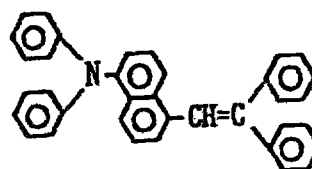
Exemplary Compound (3)-35
