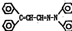
Exemplary Compound (5)-12
