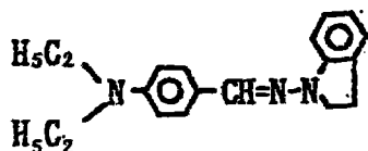
Exemplary Compound (5)-7
