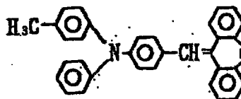
Exemplary Compound (3)-4
