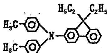
Exemplary Compound (4)-18
