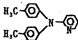
Exemplary Compound (4)-15
