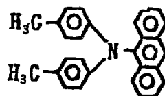
Exemplary Compound (4)-45
