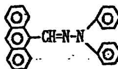
Exemplary Compound (5)-44
