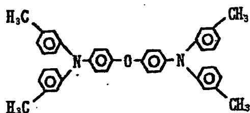
Exemplary Compound (4)-63
