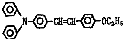
Exemplary Compound (3)-39
