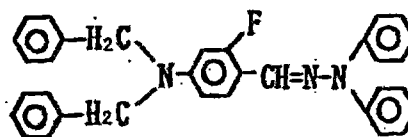
Exemplary Compound (5)-35
