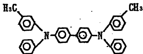
Exemplary Compound (4)-53
