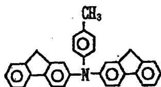
Exemplary Compound (4)-65
