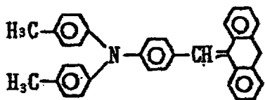
Exemplary Compound (3)-36
