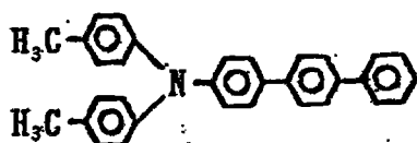
Exemplary Compound (4)-58
