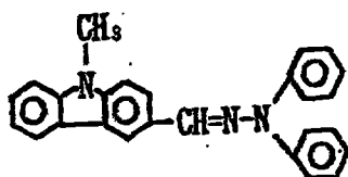
Exemplary Compound (5)-29
