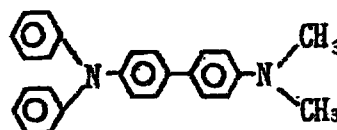
Exemplary Compound (4)-24
