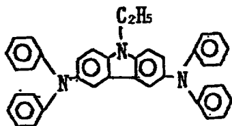
Exemplary Compound (4)-51
