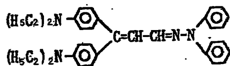
Exemplary Compound (5)-45
