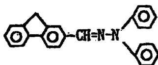
Exemplary Compound (5)-22
