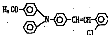
Exemplary Compound (3)-11
