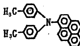
Exemplary Compound (4)-61
