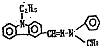
Exemplary Compound (5)-15
