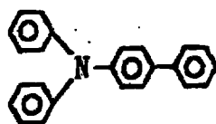
Exemplary Compound (4)-23
