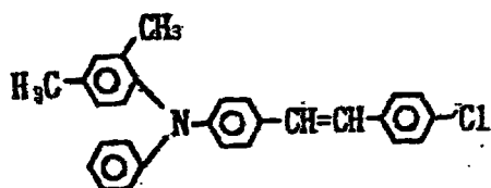
Exemplary Compound (3)-17
