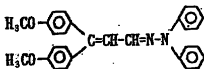
Exemplary Compound (5)-21
