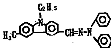
Exemplary Compound (5)-40
