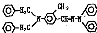
Exemplary Compound (5)-27
