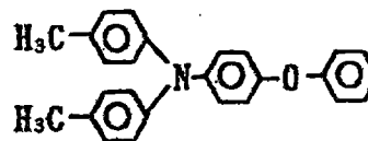
Exemplary Compound (4)-2
