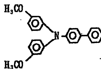
Exemplary Compound (4)-10
