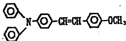
Exemplary Compound (3)-37
