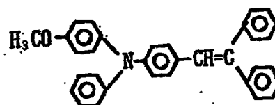
Exemplary Compound (3)-20
