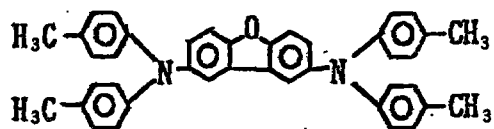
Exemplary Compound (4)-44
