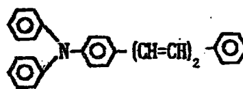
Exemplary Compound (3)-29
