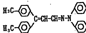
Exemplary Compound (5)-27
