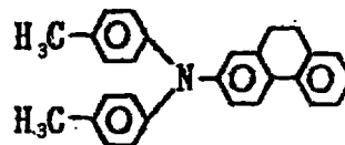
Exemplary Compound (4)-16
