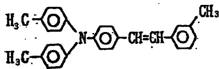
Exemplary Compound (3)-8
