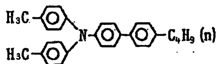
Exemplary Compound (4)-1
