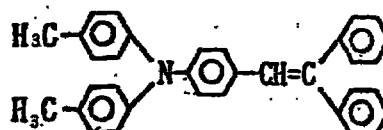
Exemplary Compound (3)-24
