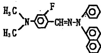
Exemplary Compound (5)-36
