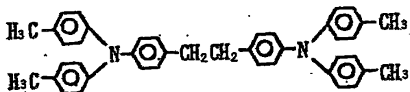
Exemplary Compound (4)-55
