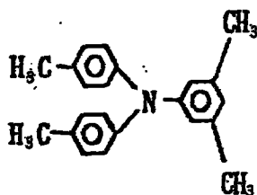
Exemplary Compound (4)-19
