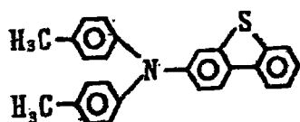
Exemplary Compound (4)-42
