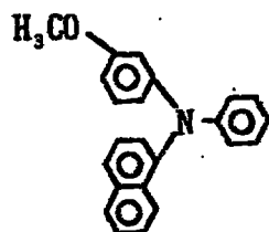
Exemplary Compound (4)-11
