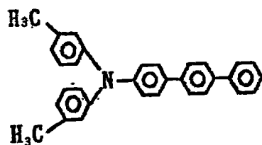
Exemplary Compound (4)-46
