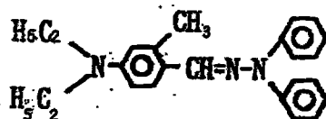
Exemplary Compound (5)-9
