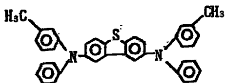
Exemplary Compound (4)-50
