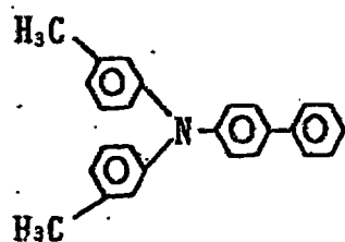
Exemplary Compound (4)-15
