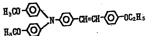
Exemplary Compound (3)-15
