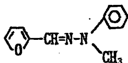
Exemplary Compound (5)-1
