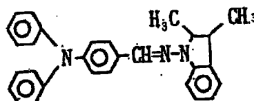
Exemplary Compound (5)-18
