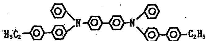
Exemplary Compound (4)-69
