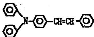
Exemplary Compound (3)-28
