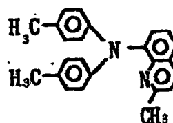
Exemplary Compound (4)-12
