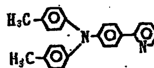
Exemplary Compound (4)-33
