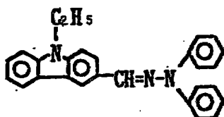
Exemplary Compound (5)-30
