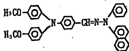
Exemplary Compound (5)-42
