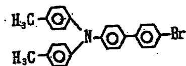
Exemplary Compound (4)-49
