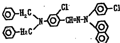
Exemplary Compound (5)-38
