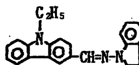
Exemplary Compound (5)-23
