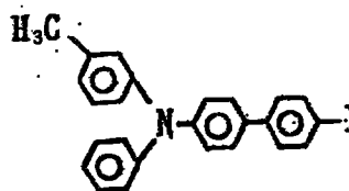
Exemplary Compound (4)-66
