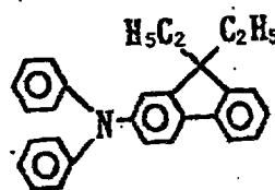
Exemplary Compound (4)-47
