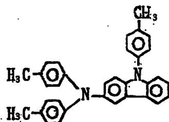
Exemplary Compound (4)-46
