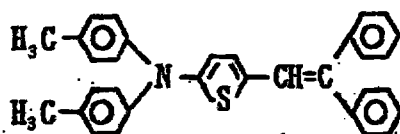
Exemplary Compound (3)-26
