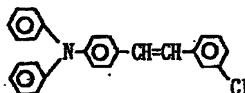
Exemplary Compound (3)-10
