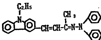
Exemplary Compound (5)-40
