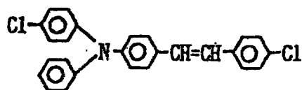
Exemplary Compound (3)-12
