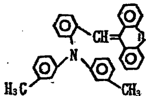
Exemplary Compound (3)-30
