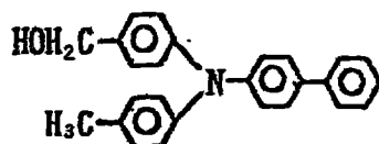
Exemplary Compound (4)-23
