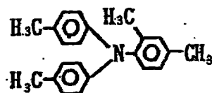
Exemplary Compound (4)-16
