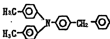
Exemplary Compound (4)-38
