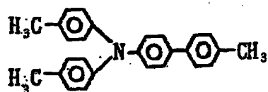
Exemplary Compound (4)-21
