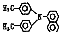
Exemplary Compound (4)-7
