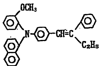
Exemplary Compound (3)-3
