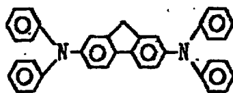
Exemplary Compound (4)-38
