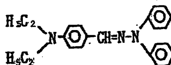
Exemplary Compound (5)-6
