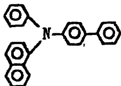
Exemplary Compound (4)-56
