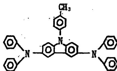
Exemplary Compound (4)-69
