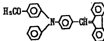
Exemplary Compound (3)-4
