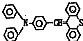
Exemplary Compound (3)-3
