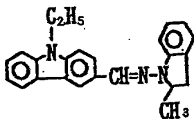
Exemplary Compound (5)-26
