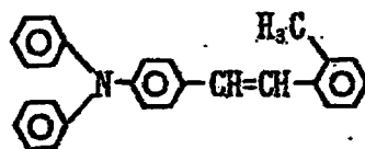
Exemplary Compound (3)-7
