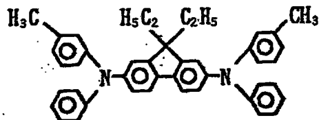
Exemplary Compound (4)-56
