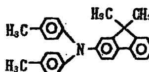
Exemplary Compound (4)-71
