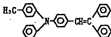
Exemplary Compound (3)-7
