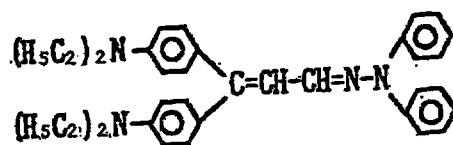
Exemplary Compound (5)-37
