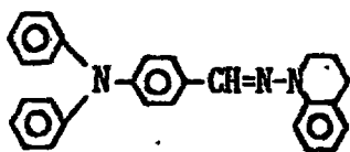
Exemplary Compound (5)-32
