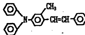
Exemplary Compound (3)-27
