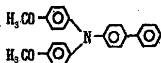
Exemplary Compound (4)-30
