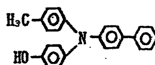
Exemplary Compound (4)-31
