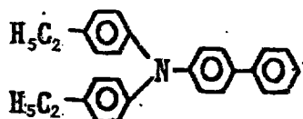
Exemplary Compound (4)-3
