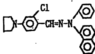
Exemplary Compound (5)-37
