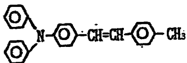
Exemplary Compound (3)-36
