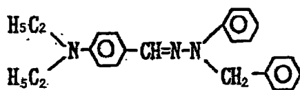
Exemplary Compound (5)-15
