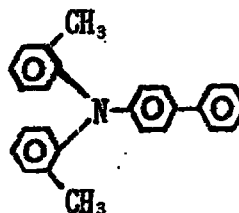
Exemplary Compound (4)-24
