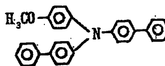
Exemplary Compound (4)-41
