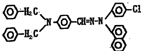
Exemplary Compound (5)-21
