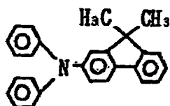
Exemplary Compound (4)-70
