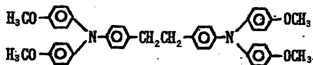
Exemplary Compound (4)-42
