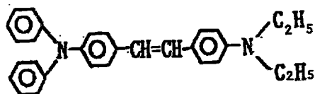
Exemplary Compound (3)-13
