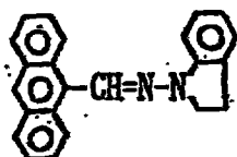
Exemplary Compound (5)-43
