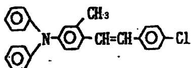
Exemplary Compound (3)-19
