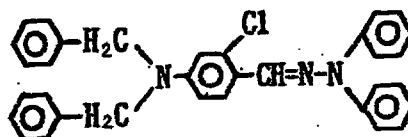
Exemplary Compound (5)-33
