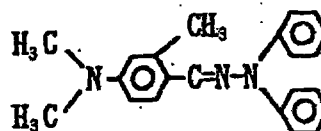
Exemplary Compound (5)-20
