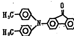
Exemplary Compound (4)-37
