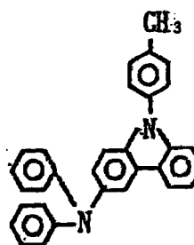
Exemplary Compound (4)-41
