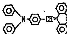
Exemplary Compound (3)-6
