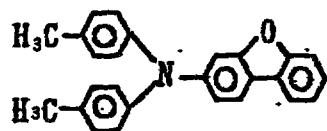
Exemplary Compound (4)-50
