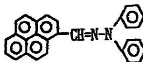
Exemplary Compound (5)-18
