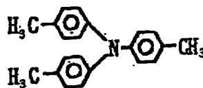
Exemplary Compound (4)-22
