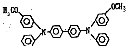
Exemplary Compound (4)-35
