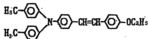
Exemplary Compound (3)-22
