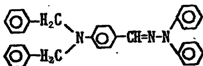
Exemplary Compound (5)-28
