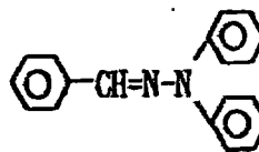
Exemplary Compound (5)-16
