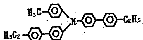
Exemplary Compound (4)-27
