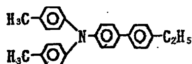
Exemplary Compound (4)-4
