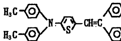
Exemplary Compound (3)-33
