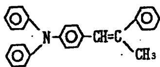
Exemplary Compound (3)-32
