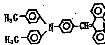
Exemplary Compound (3)-40
