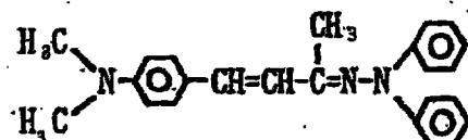
Exemplary Compound (5)-11
