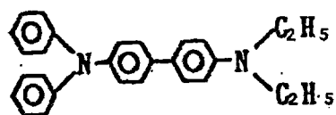
Exemplary Compound (4)-25
