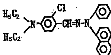
Exemplary Compound (5)-19
