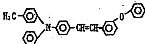
Exemplary Compound (3)-26
