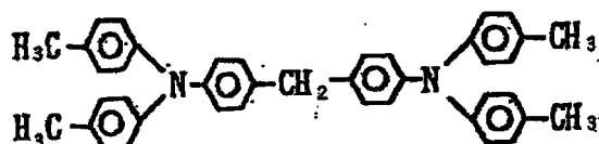
Exemplary Compound (4)-68
