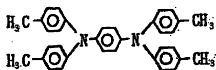
Exemplary Compound (4)-67
