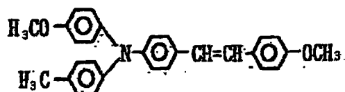
Exemplary Compound (3)-14
