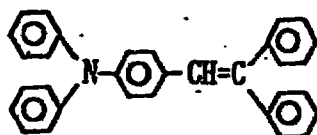
Exemplary Compound (3)-9
