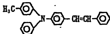
Exemplary Compound (3)-23
