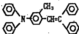
Exemplary Compound (3)-16
