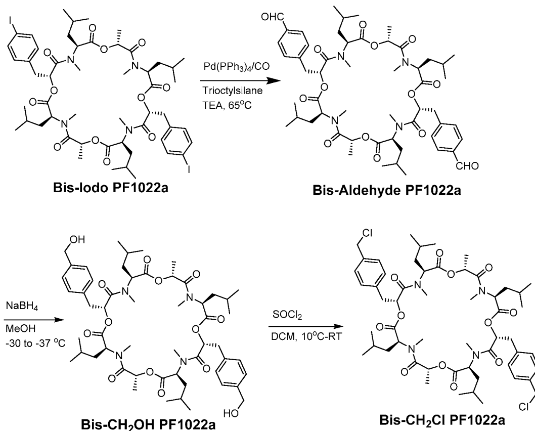
Scheme 1c: Route for Preparation of Bis-CH 2 Cl PF1022a:
