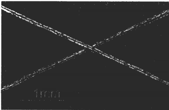
SPECIMEN III PRESENT INVENTION epoxy primer 2000 hours FIG. 1a
