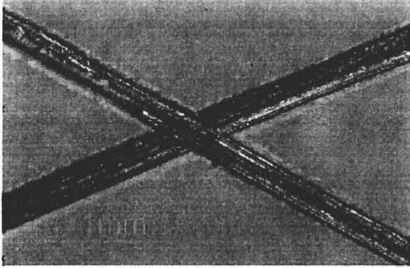
SPECIMEN II SrCrO 4 epoxy primer (hexavalent chromium) 2000 hours FIG. 1c
