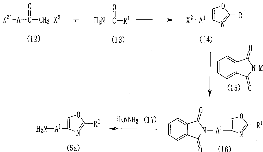
Reaction Scheme 10
