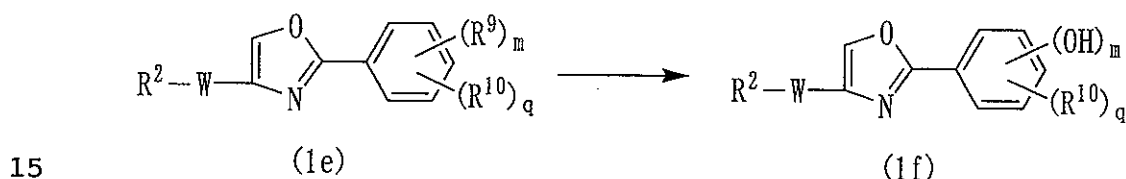
Reaction Scheme 5
