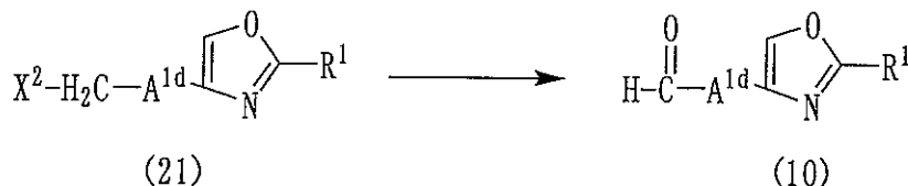
Reaction Scheme 12
