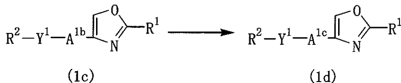
Reaction Scheme 4
