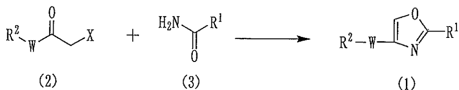
Reaction Scheme 1
