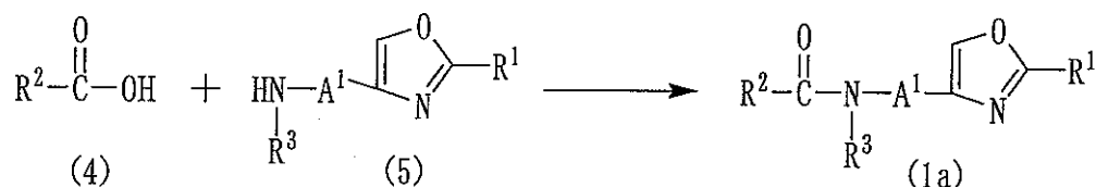
Reaction Scheme 2
