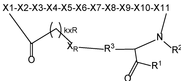
Formula (I-1),
