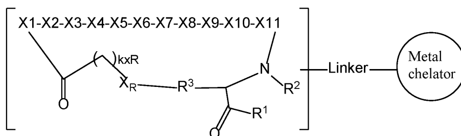
Formula (III-1),
