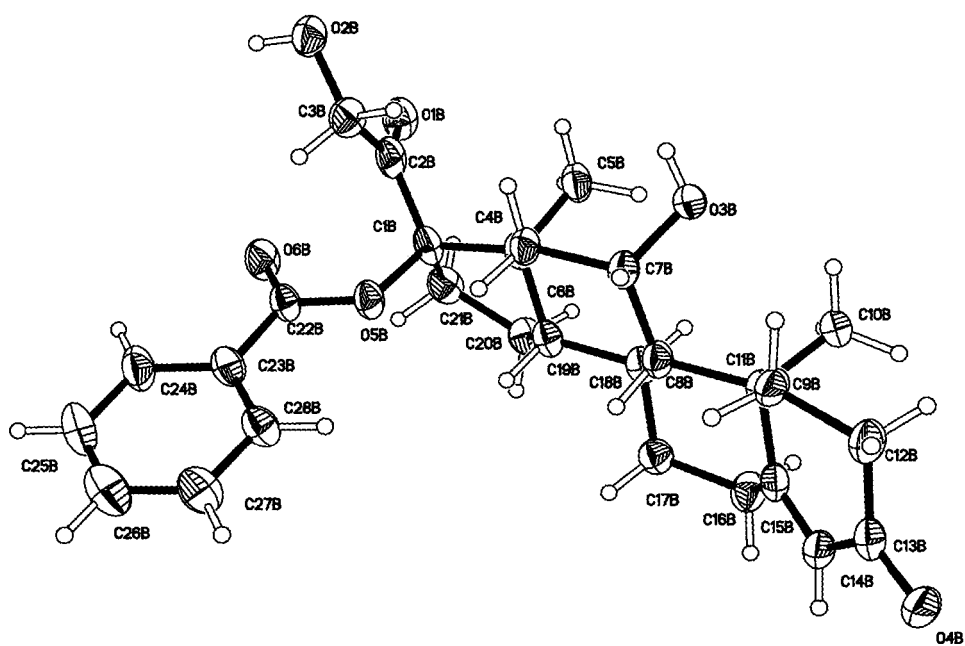
Molecule B
