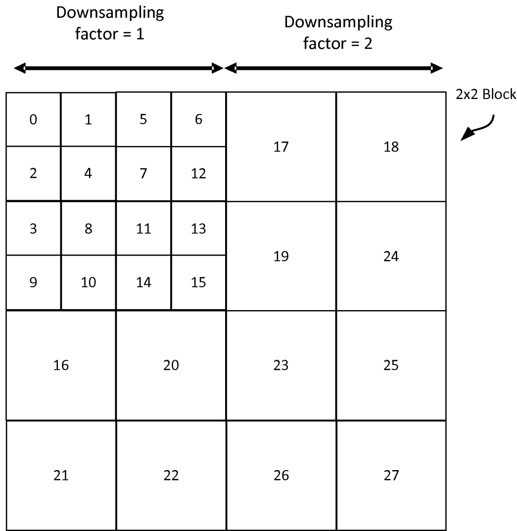
Non-uniform sampling for a 8x8 quantization matrix
