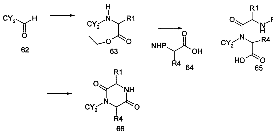
Scheme 15
