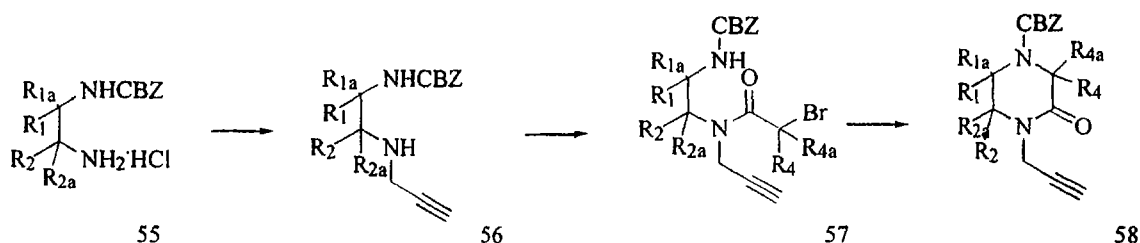
Scheme 12
