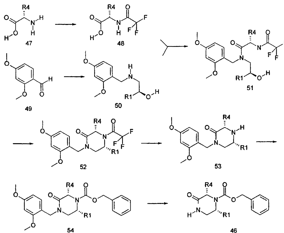
Scheme 11
