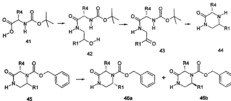
Scheme 10.
