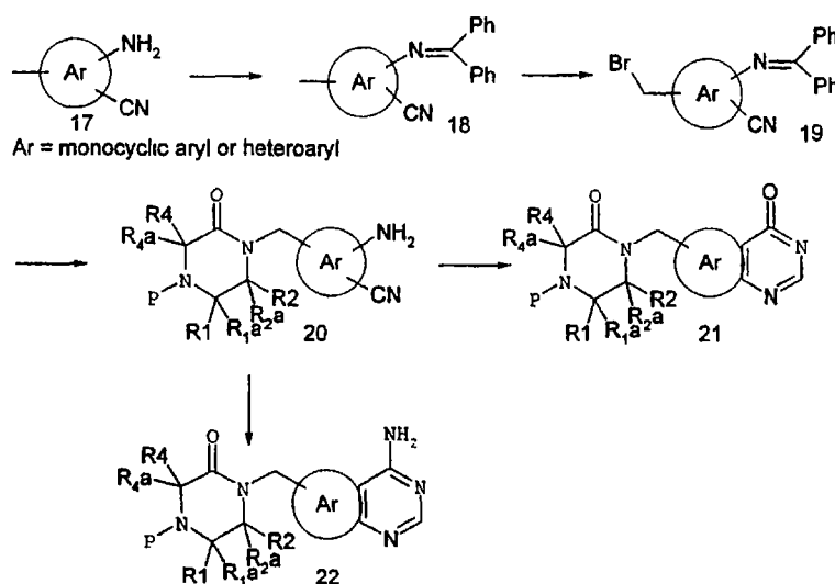
Scheme 6.
