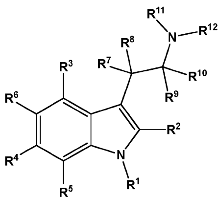
Formula (I-J)
