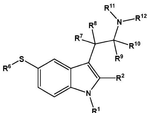
Formula (I-C)
