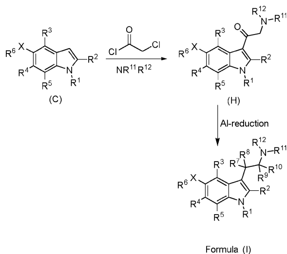
Scheme VII
