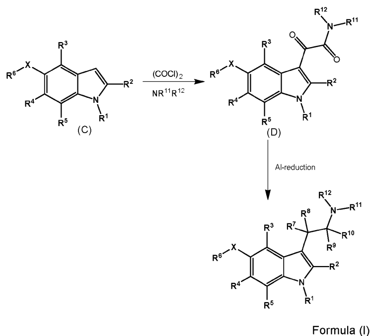
Scheme II
