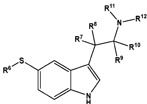
Formula (I-F)
