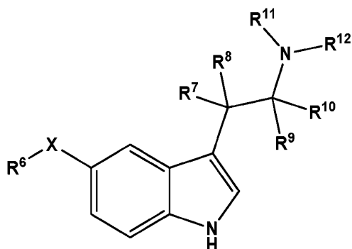
Formula (I-E)
