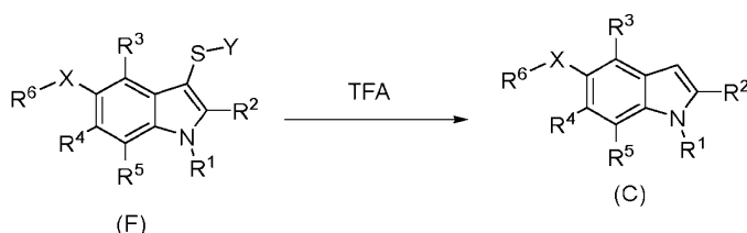
Scheme IV
