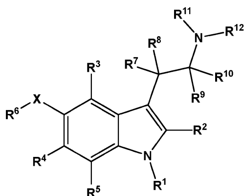
Formula (I-H)
