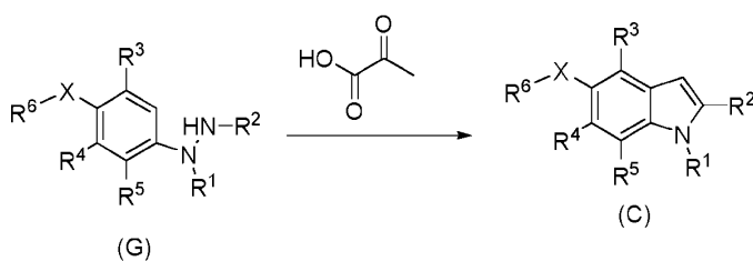
Scheme V
