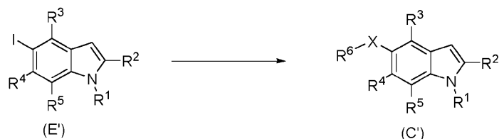
Scheme IX
