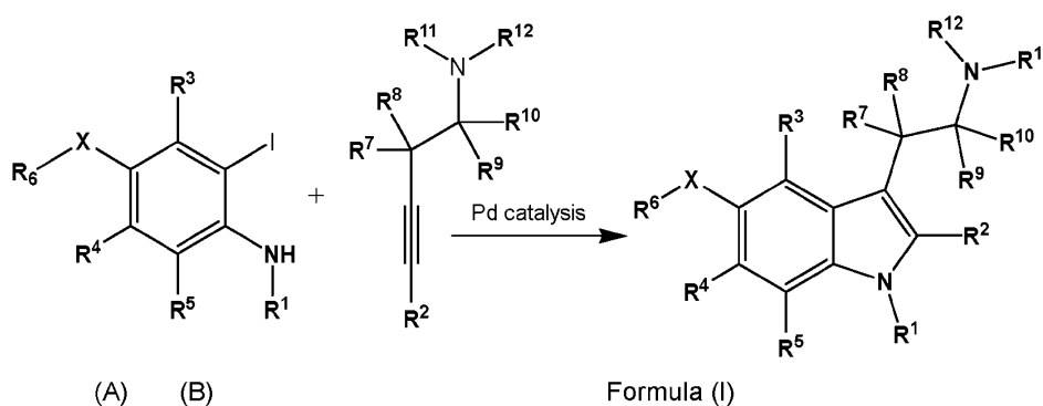
Scheme I
