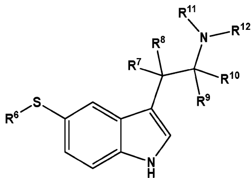
Formula (I-D)
