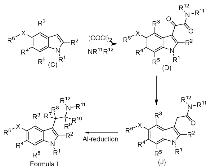
Scheme VIII
