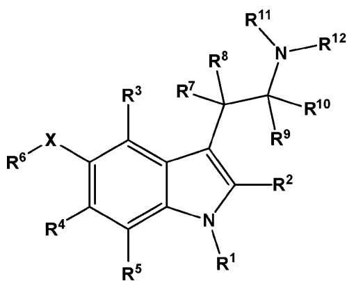
Formula (I-G)
