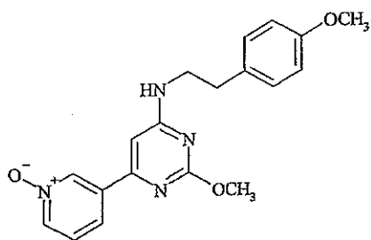
[2-methoxy-6-(1-oxy-pyridin-3-yl)-pyrimidin-4-yl]-[2-(4-methoxy-phenyl)-ethyl]-amine.
