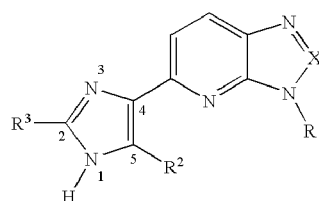
1H-Imidazole Tautomer I
