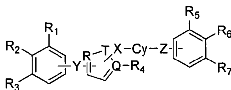
(formula IV)
