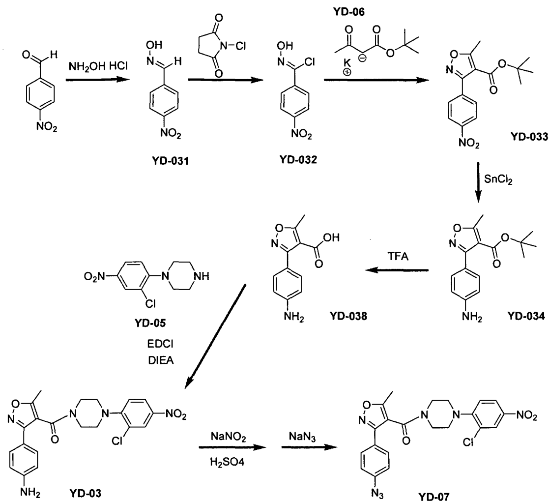
Scheme 3. Synthesis of Compound 3 (YD-03) and Compound 4 (YD-07)
