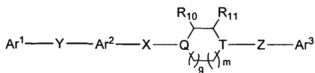
(formula V)
