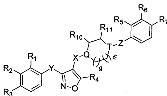
(formula VI)
