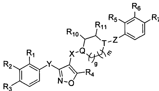
(formula VI)
