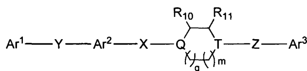
(formula V)
