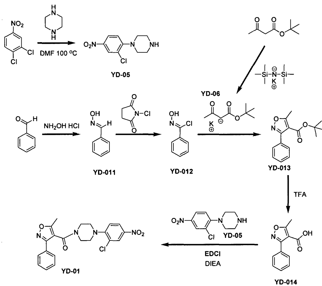
Scheme 2. The synthesis of compound 2 (YD-01):
