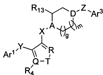
(formula III)
