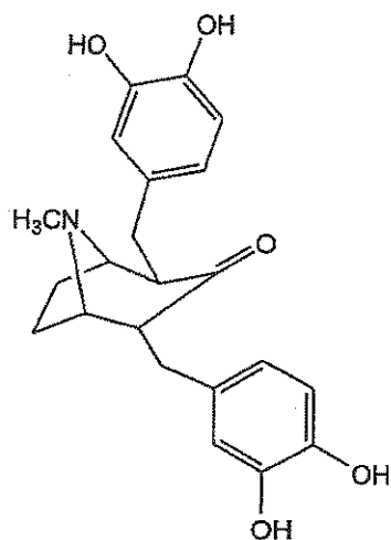
2,4-bis(3,4-dihydroxybenzyl)-8-methyl -8-aza-bicyclo[3.2.1]octan-3-one
