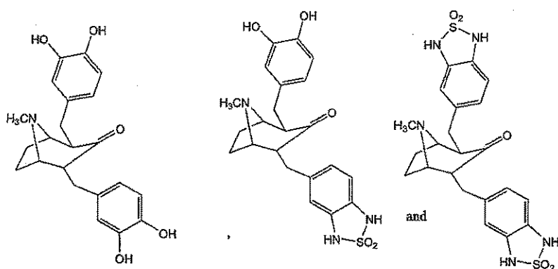
2,4-bis(3,4-dihydroxybenzyl)-8-methyl-8-aza-bicyclo[3.2.1]octan-3-one
