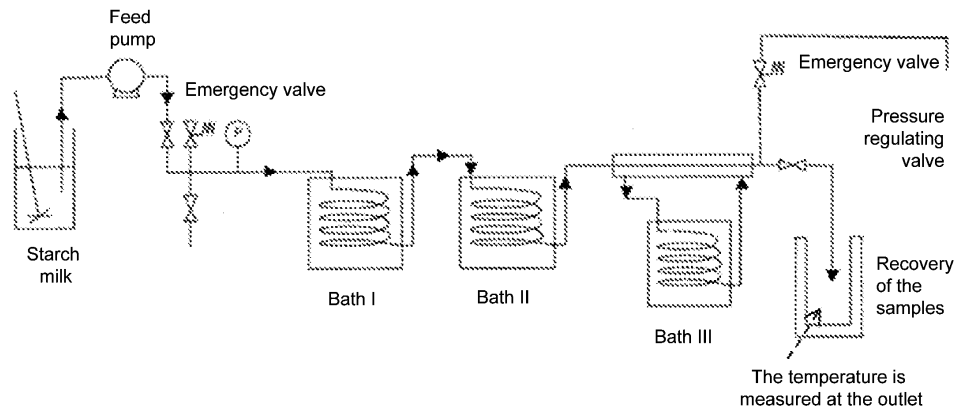
Continuous reactor
