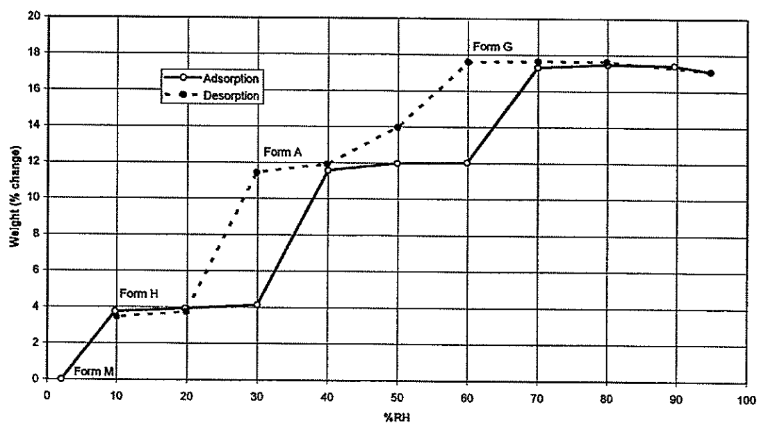
Figure 1 Sorption results of Modification A
