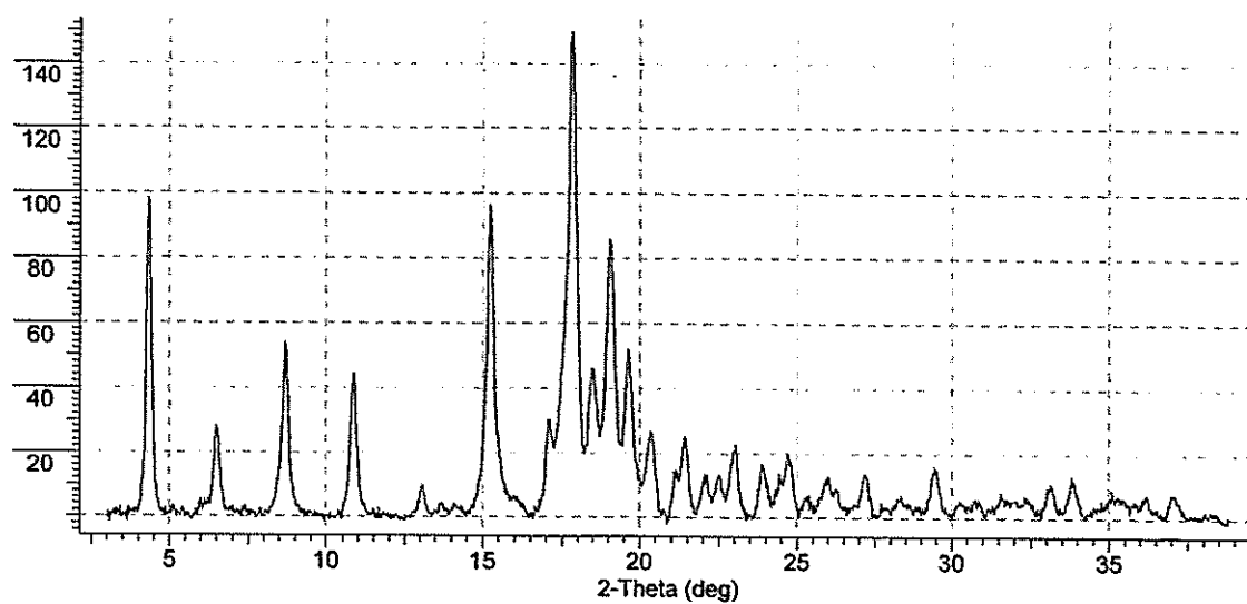
5 Figure 2.16 X-ray Powder Diffraction Pattern (PXRD) of Modification P
