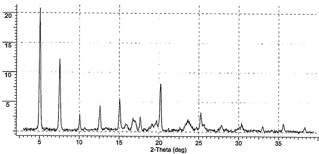
5 Figure 2.4: X-ray Powder Diffraction Pattern (PXRD) of Modification D
