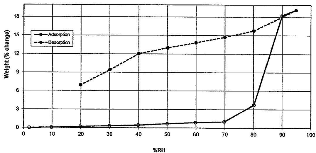
5 Figure 6 Sorption profile at 25°C of Modification N
