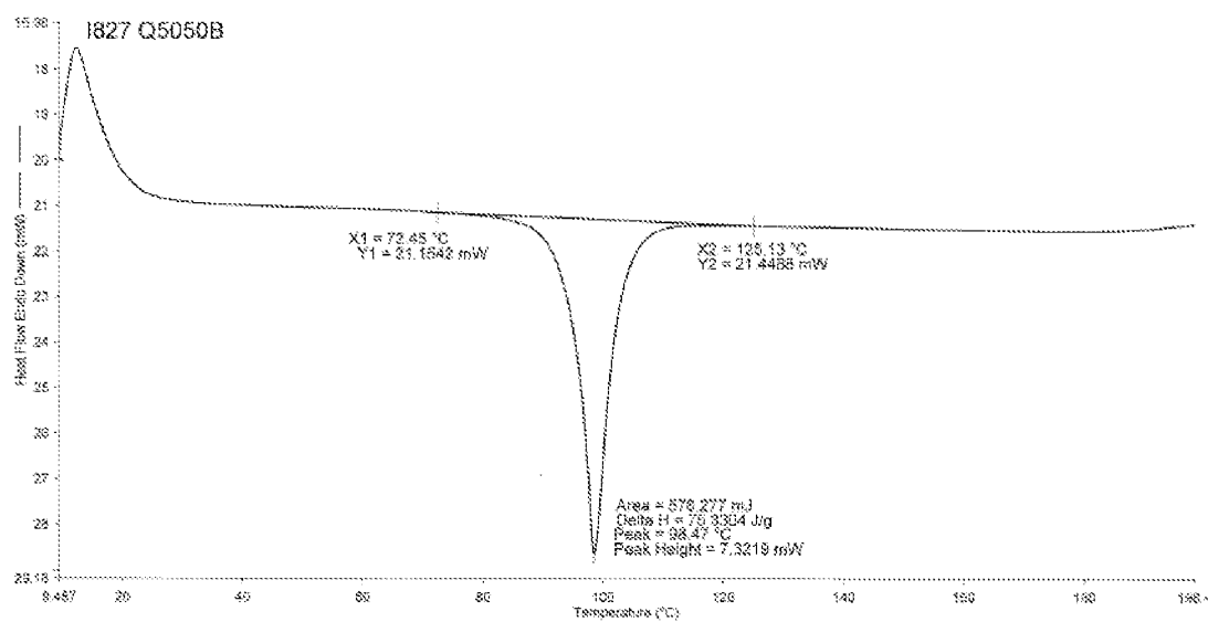
FIG. 7 DSC of Formula IVa, Form II
