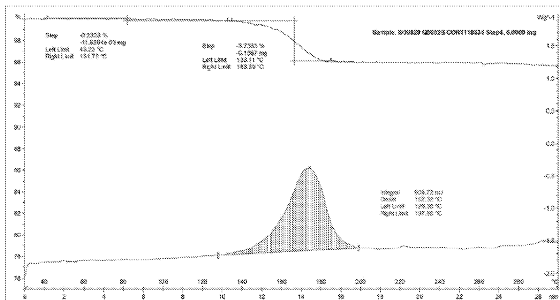
FIG. 3 TGA of Formula II Monohydrate
