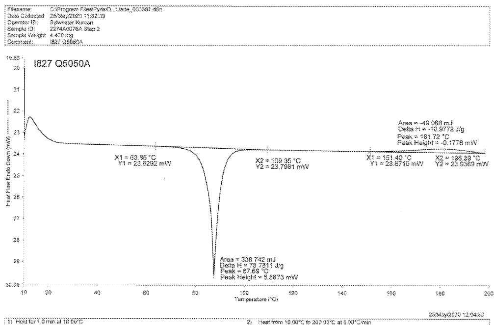
FIG. 5 DSC of Formula IVa, Form I
