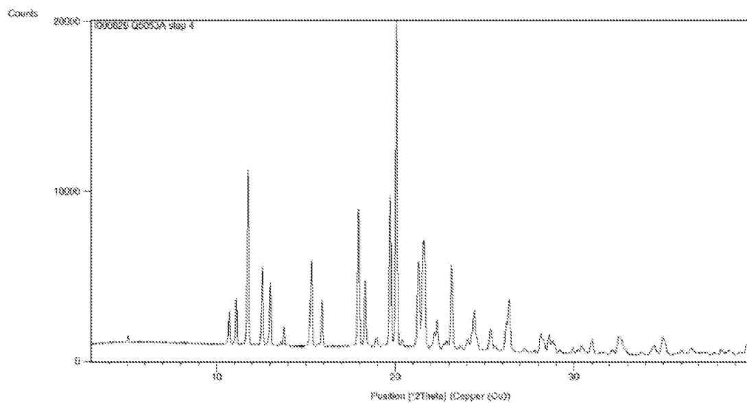
FIG. 1 XRPD of Formula II Monohydrate
