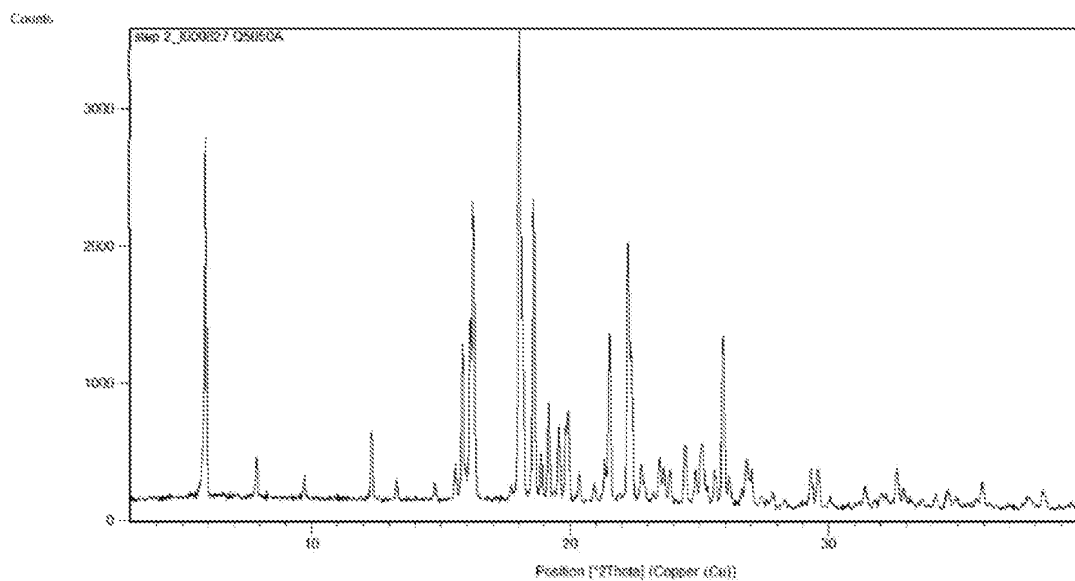
FIG. 4 XRPD of Formula IVa, Form I
