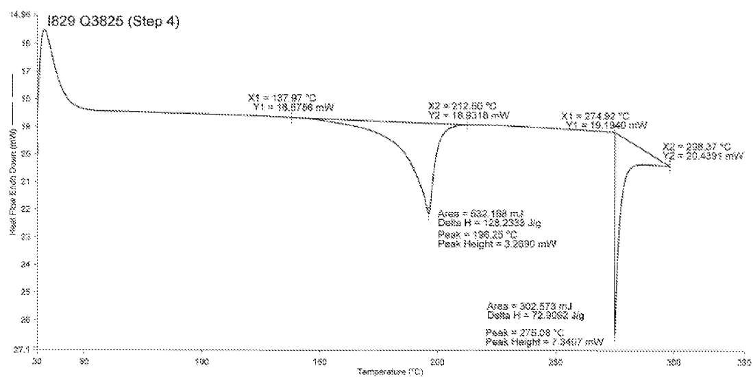
FIG. 2 DSC of Formula II Monohydrate
