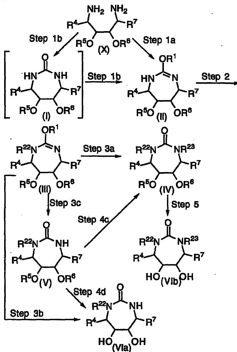
10 Scheme 6.
