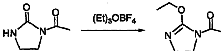
25 Scheme 2.
