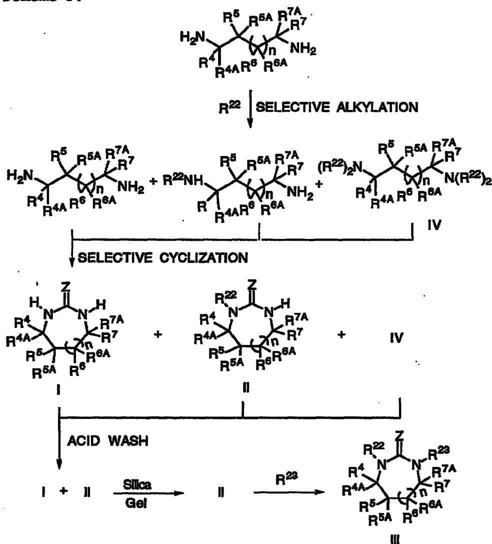
Scheme 3.
