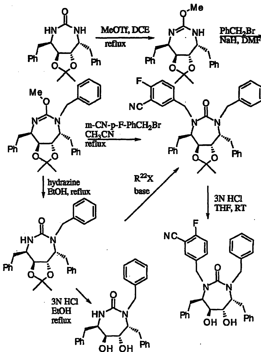
Scheme 7.
