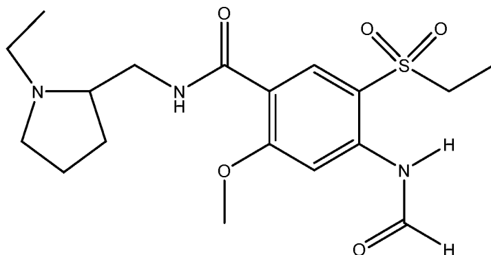
Compound 1
