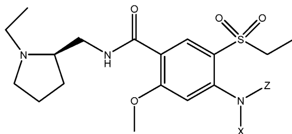
Formula IA-S
