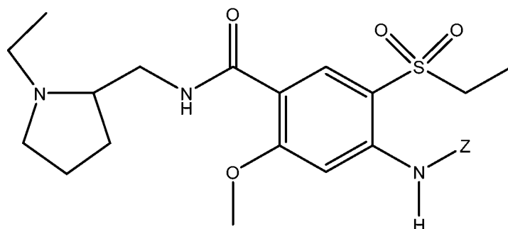
Formula IB
