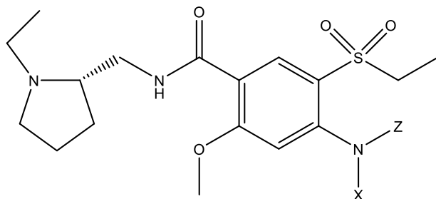
Formula IA-R
