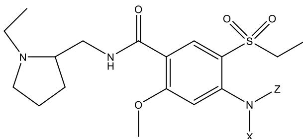
Formula IA
