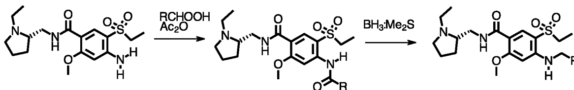
Scheme 3. Preparation of Amisulpride Derivatives ( S -Isomer as an example)
