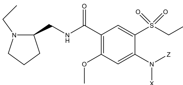
Formula IA-S
