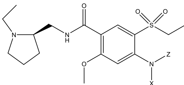
Formula IA-S
