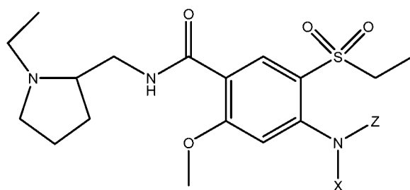
Formula IA
