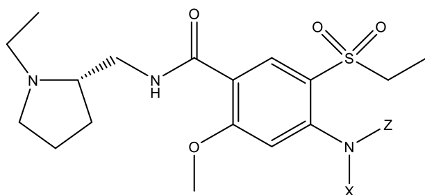
Formula IA-R
