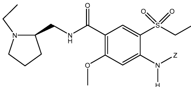
Formula IB-S
