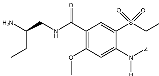
Formula IC-S
