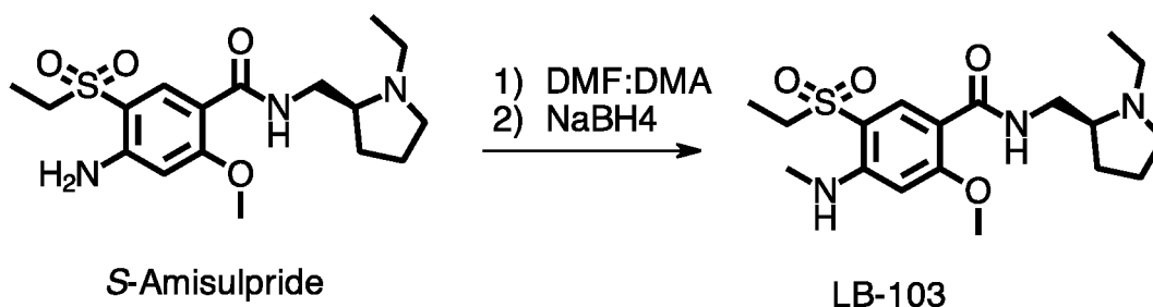
Scheme 4. Preparation of 4-Methylamino Substituted Amisulpride Derivatives ( S -Isomer)
