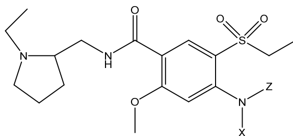
Formula IA
