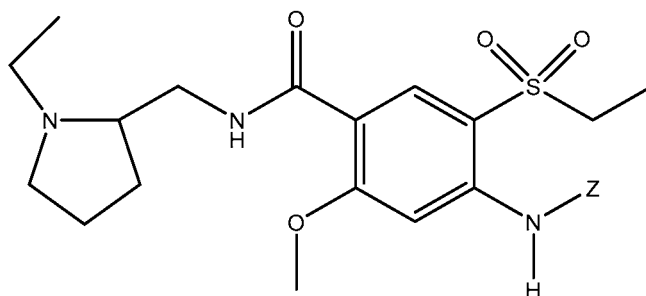
Formula IB
