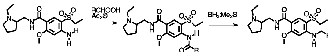
Scheme 1. Preparation of Amisulpride Derivatives
