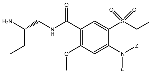
Formula IC-R
