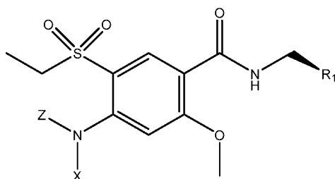
Formula I-S
