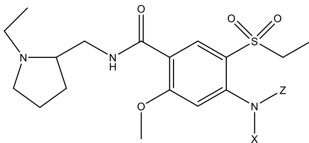
Formula IA
