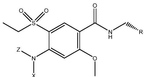
Formula I-R
