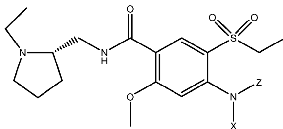
Formula IA-R
