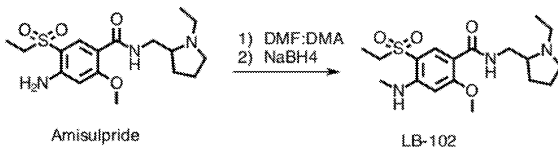
Scheme 2. Preparation of 4-Methylamino Substituted Amisulpride Derivatives
