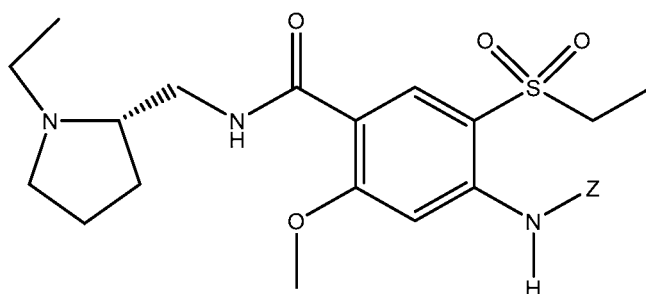
Formula IB-R
