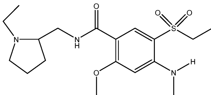
Compound 102
