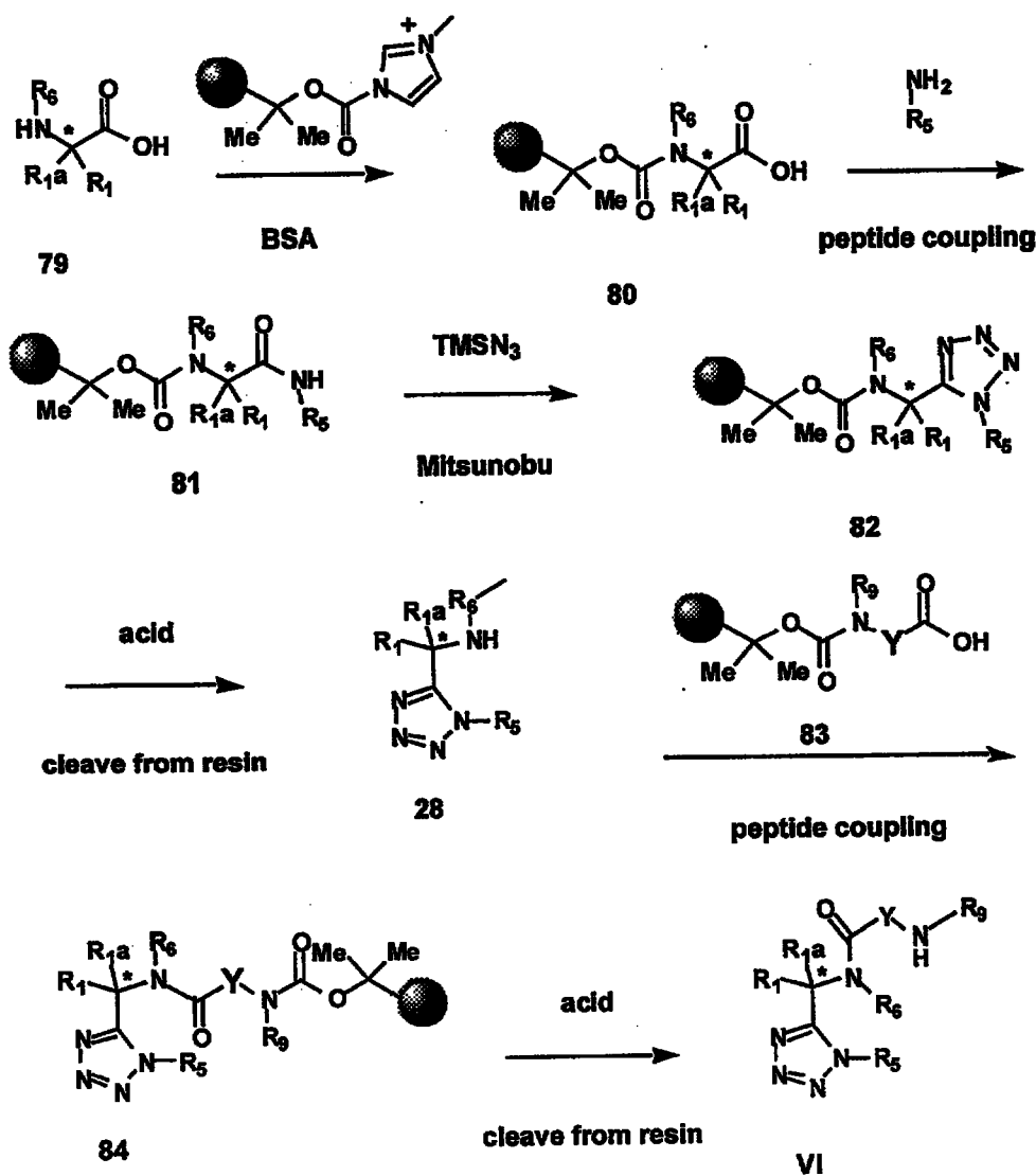
Scheme 6:
