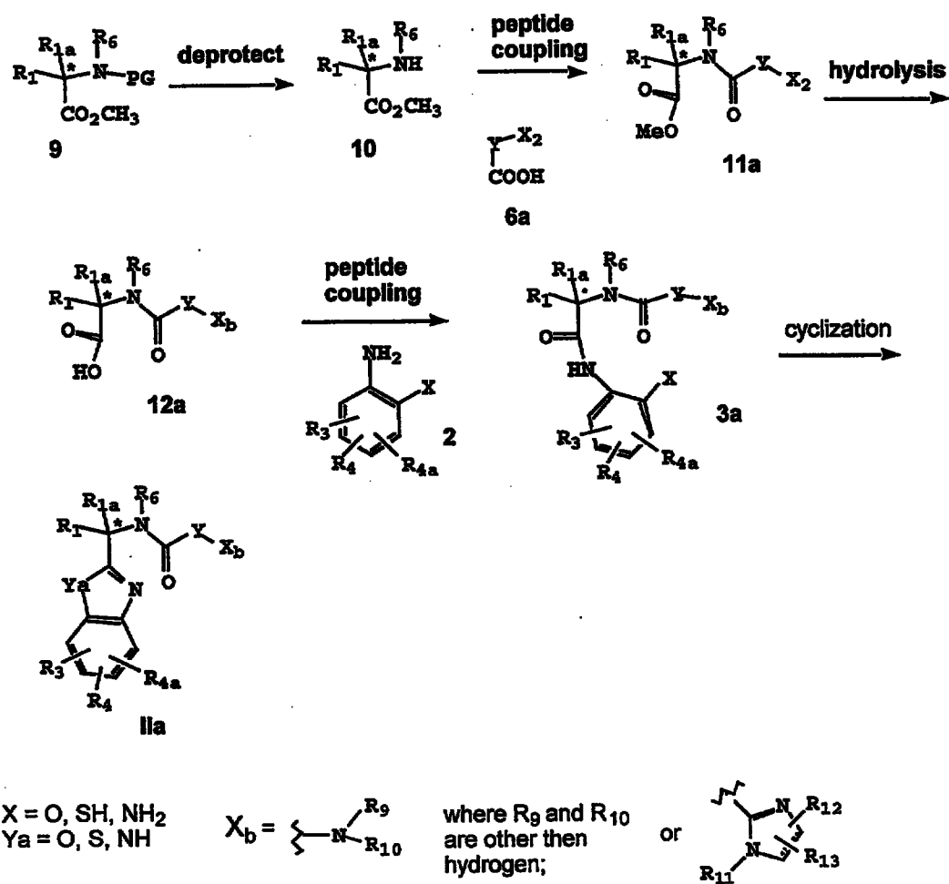
Scheme 1b
