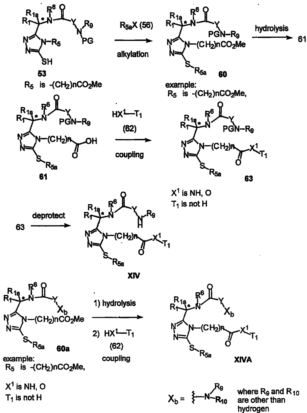
Scheme 4d
