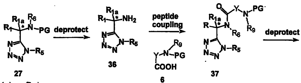
Scheme 3b
