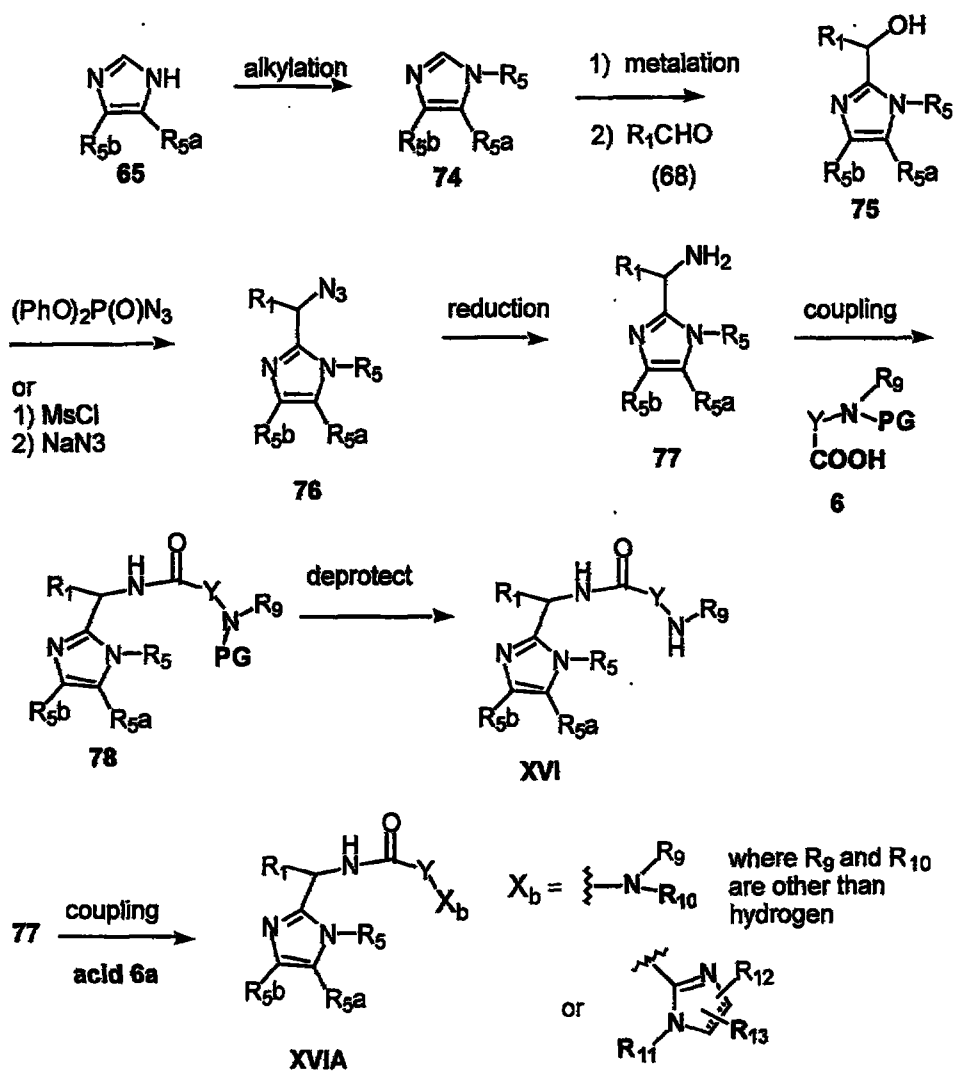
Scheme 5a
