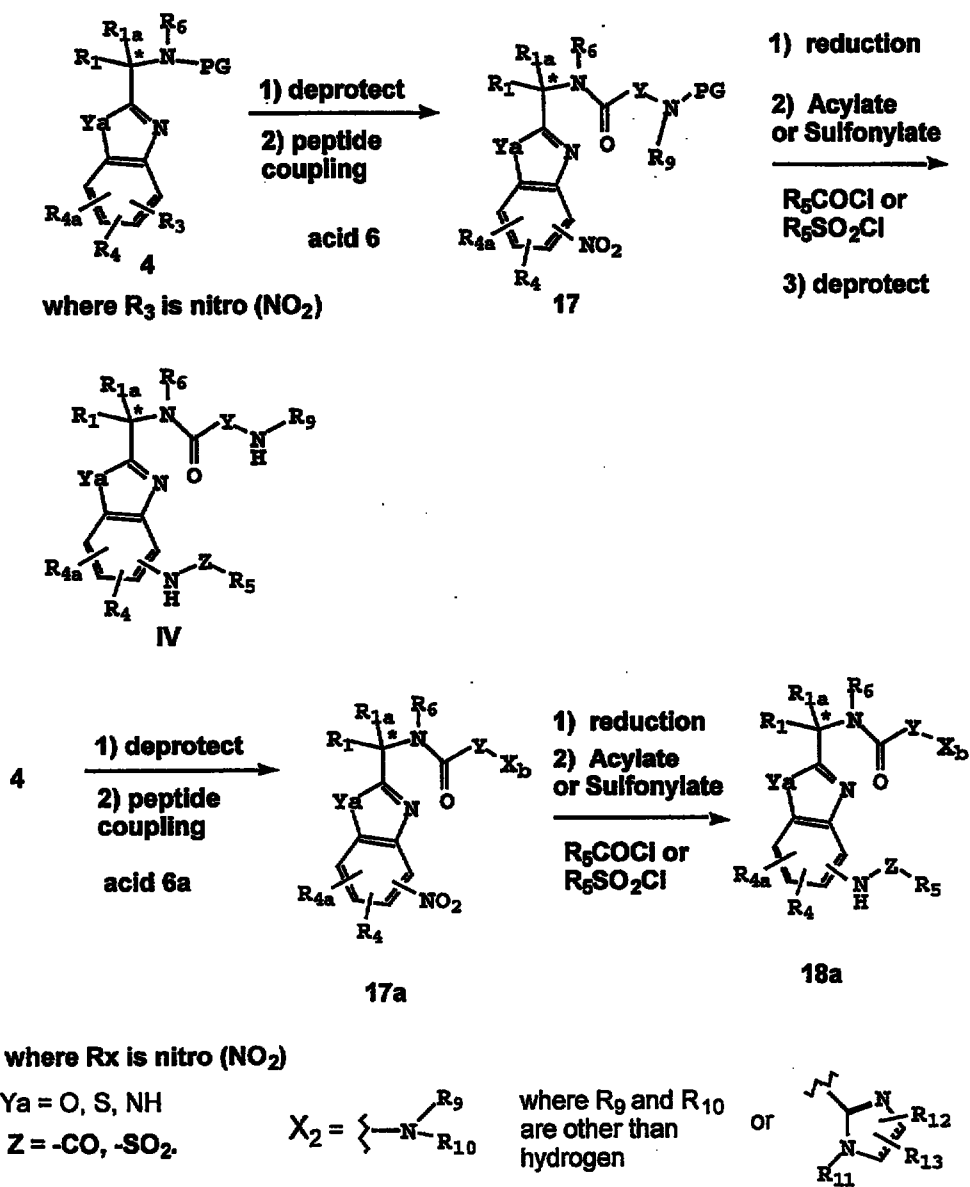
Scheme 1d
