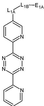
Formula (1); wherein
