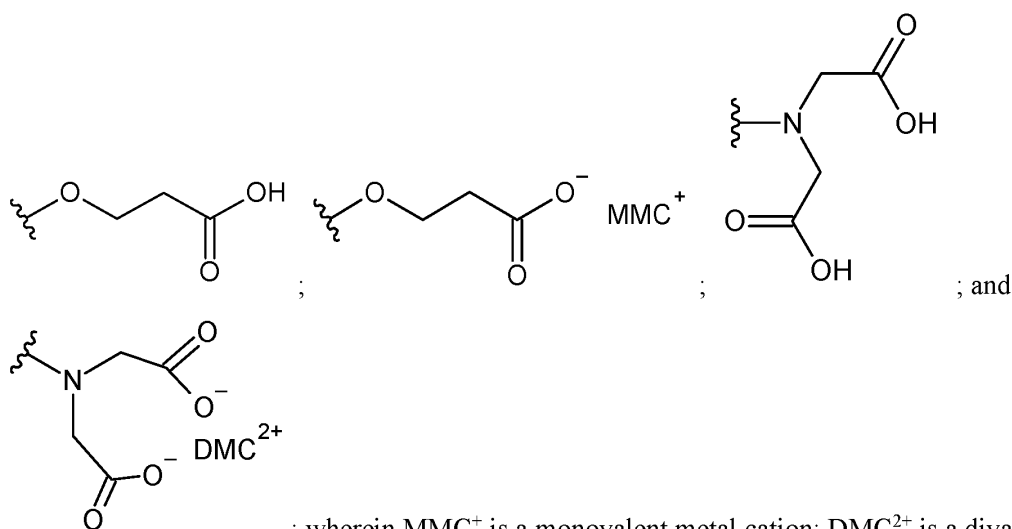
Formula (1); wherein
