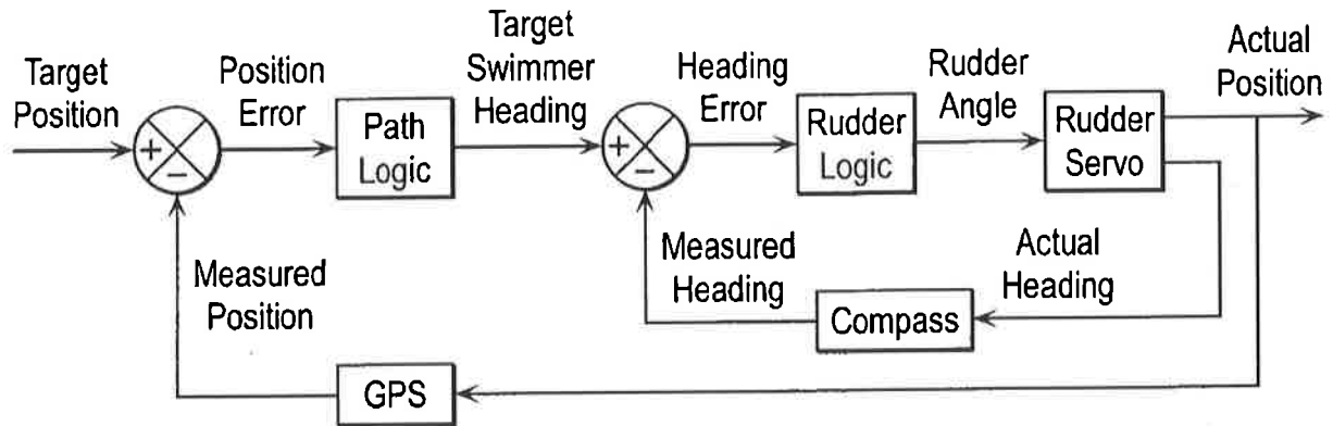
FIG. 13 (Prior Art)
