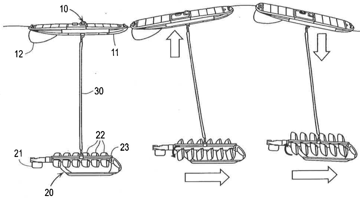
FIG. 1 (Prior Art)
