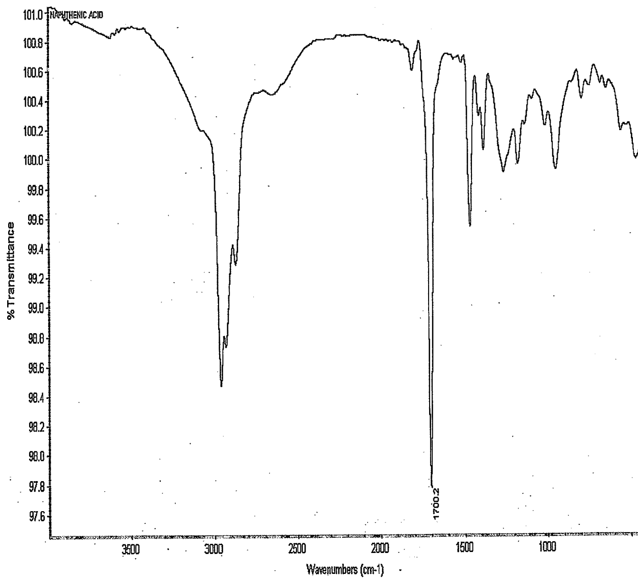
Fig.1: FTIR spectrum of naphthenic acid
