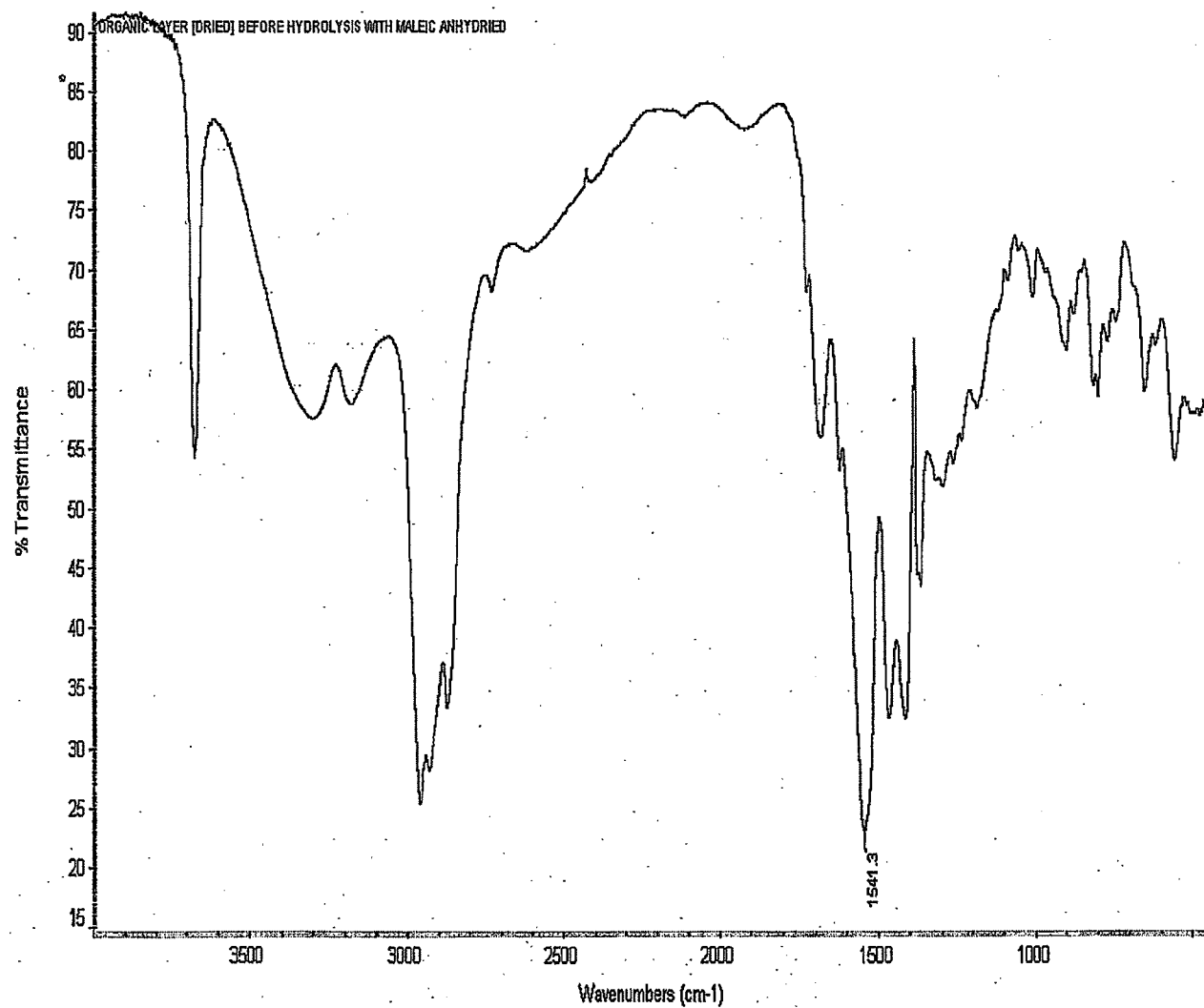
Fig.3: FTIR spectrum of Organic layer [Ca-naphthenate in toluene (oven dried)] before reaction
