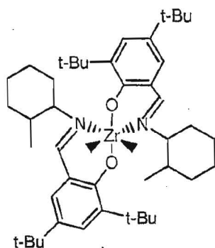
Catalyst A2
