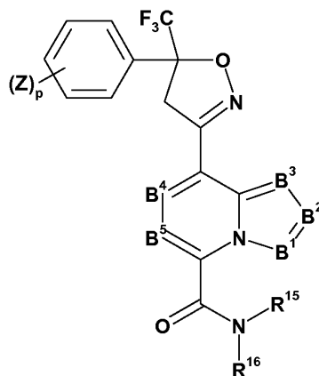
Formula (IV)
