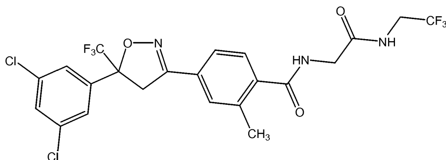
Compound B
