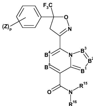
Formula (III)
