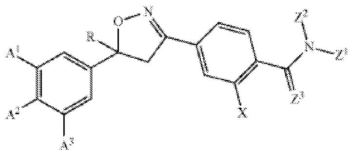
Formula (II)
