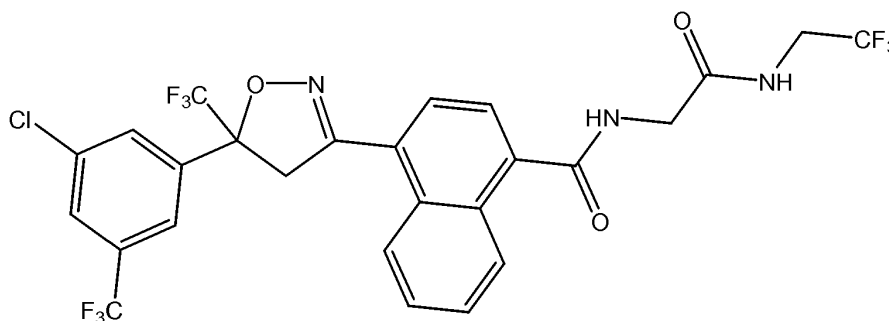
Compound A
