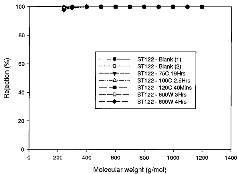
Figure 1: Rejection performance of Starmem™ 122 membranes operated at 30bar and 30°C having been subjected to thermal and microwave curing cycles. Toluene flux for these membranes is presented in Table 3, Entries 1-7.
