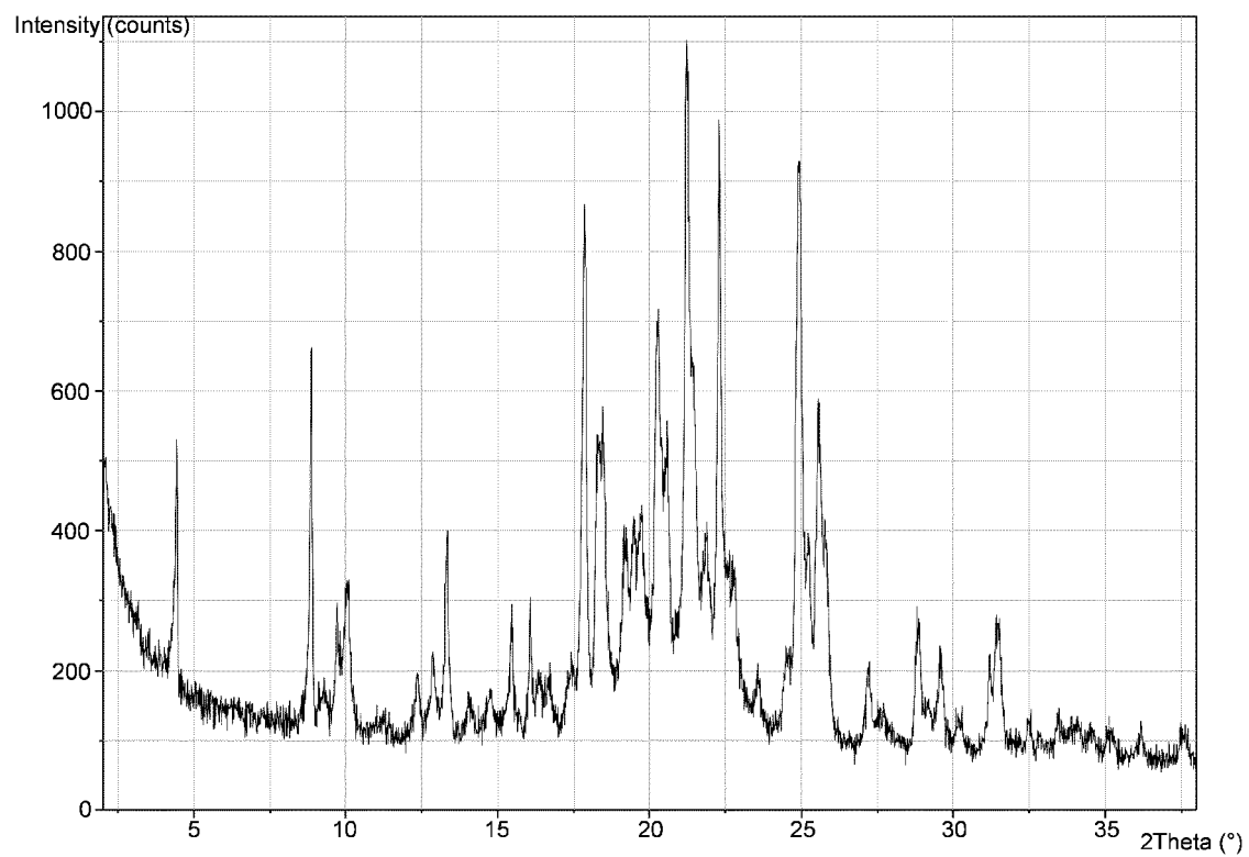
FIGURE 1 X-Ray powder diffractogram of polymorphic form B of compound of formula (I)
