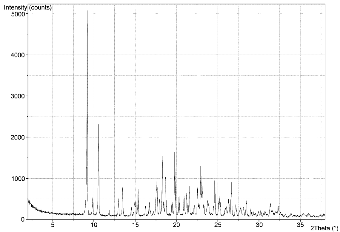
FIGURE 3: X-Ray powder diffractogram of 1,7-hydrate of compound of formula (I)
