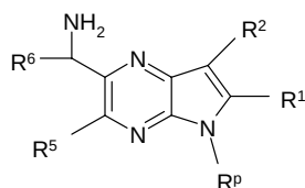
Formula 3
