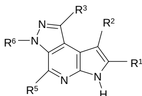
Formula (Ig)
