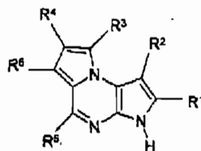
Formula (1d)
