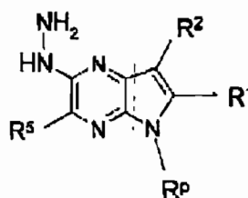
Formula 2
