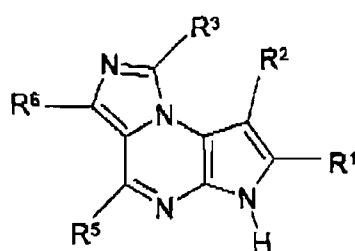
Formula (Ib)
