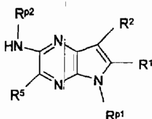
Formula 4
