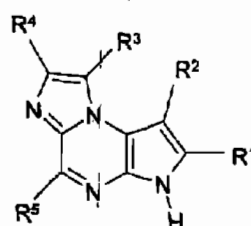
Formula (1c)
