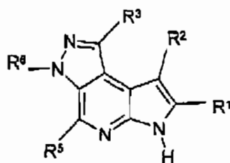
Formula (Ig)
