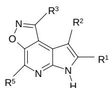
Formula (If) .
