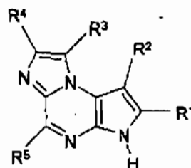
Formula (1c)
