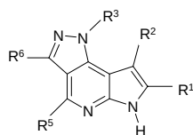
Formula (Ie) .
