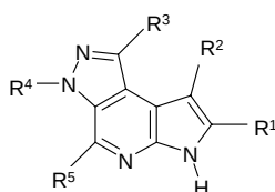
Formula (Ig)
