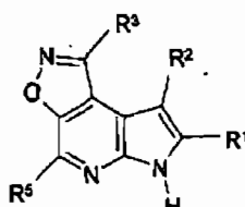
Formula (If)
