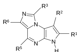
Formula (Ib)
