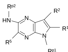
Formula 4
