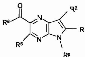
Formula 5
