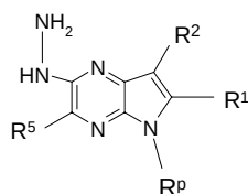
Formula 2
