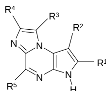
Formula (Ic)
