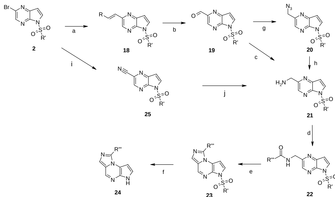
Scheme IV
