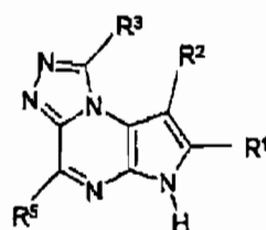
Formula (1a)
