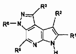
Formula (Ig)
