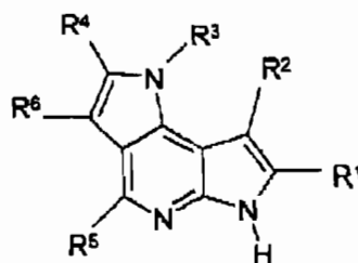
Formula (Ih)
