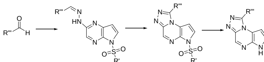
Scheme 7. Formation of a hydrazone followed by cyclization and sulfonamide hydrolysis (General Procedure G)
