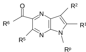
Formula 5
