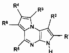
Formula (Id)
