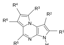
Formula (Id)
