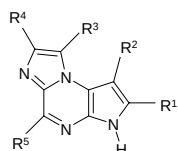
Formula (Ic)
