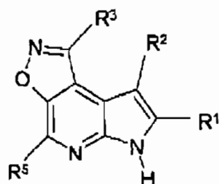
Formula (If)
