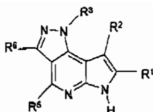
Formula (Ie)
