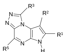
Formula (Ia)
