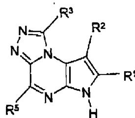
Formula (Ia)
