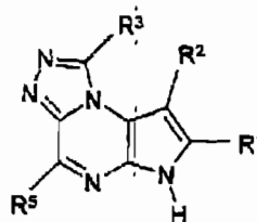
Formula (Ia)
