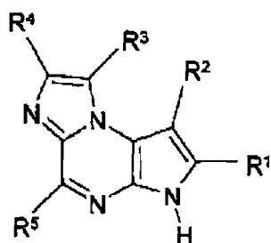
Formula (Ic)
