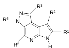
Formula (Ig) .
