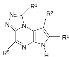
Formula (Ia)
