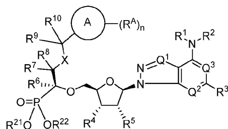
Formula (Ib).
