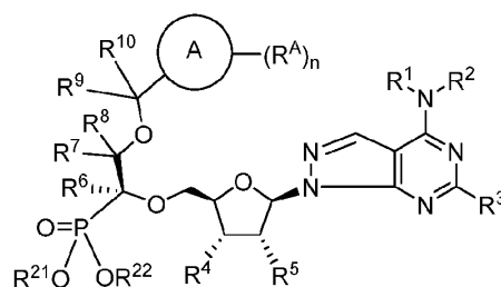
Formula (Ic).
