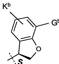
(S)-(Fb7)
