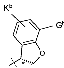
(R)-(Fb7)*
