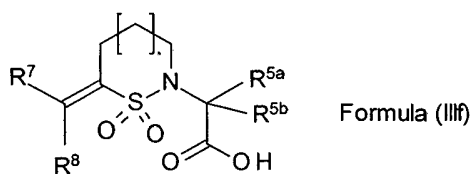
Scheme 9-1:
