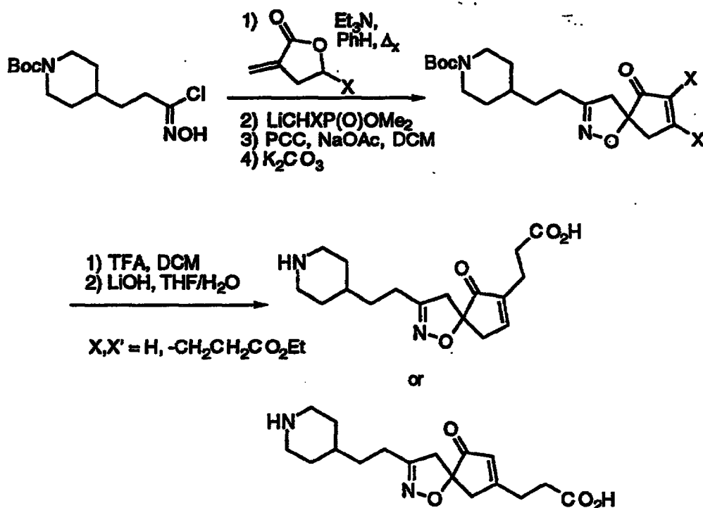
Scheme VII
