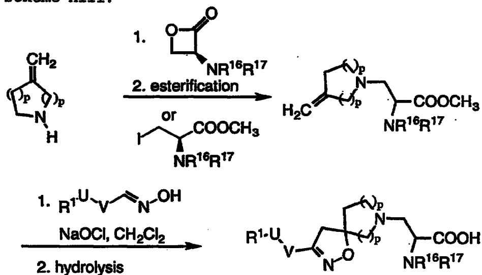
Scheme XIII.
