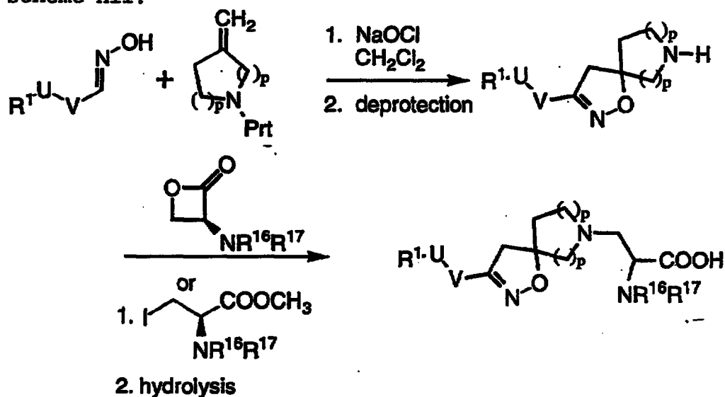
Scheme XII.
