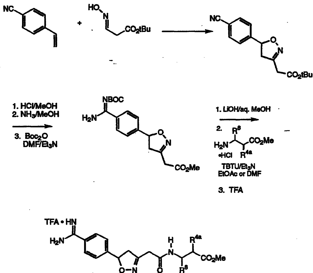
Scheme 1b
