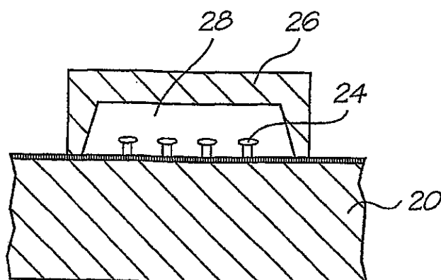
FIG. 3 (Prior Art)
