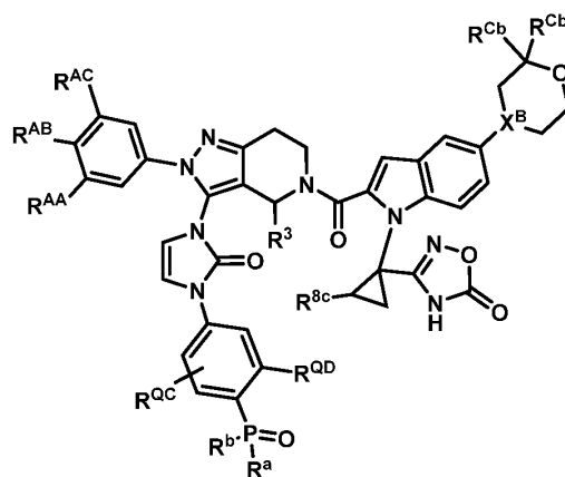
Formula (IE)
