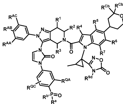
Formula (ID)
