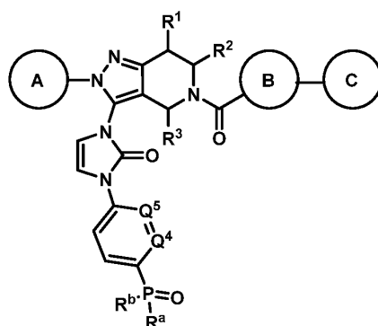
Formula (IA)
