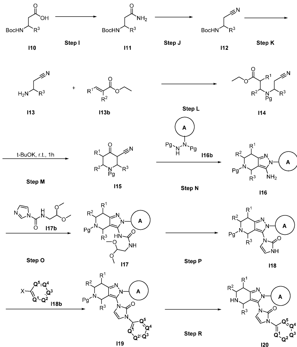
Scheme 2
