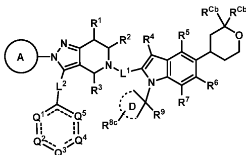
Formula (IC)
