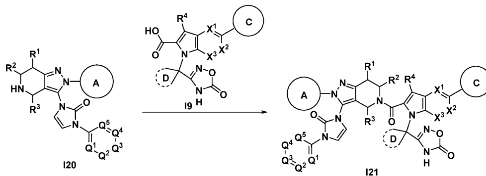
Scheme 3
