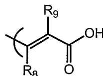
" trans -cinnamic acid"
