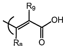
"trans-cinnamic acid"
