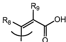
"cis-cinnamic acid"
