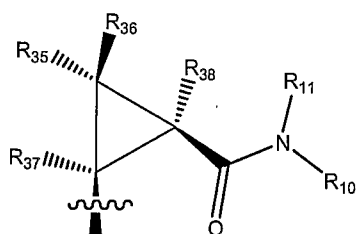
" cis -cyclopropanamide"
