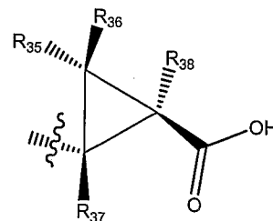
"trans-cyclopropanoic acid"
