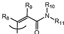
"cis-cinnamide"
