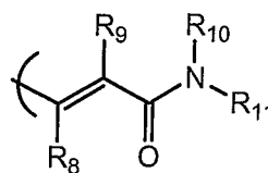
" trans -cinnamide"
