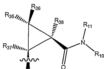
"cis-cyclopropanamide"
