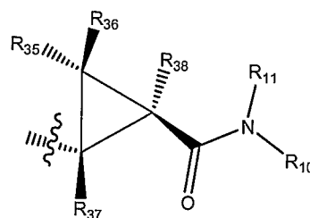
"trans-cyclopropanamide"
