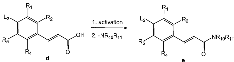
Scheme 2
