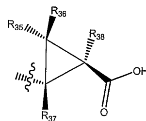
"trans-cyclopropanoic acid"
