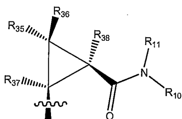
"cis-cyclopropanamide"
