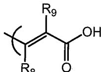
"trans-cinnamic acid"
