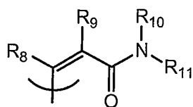
" cis -cinnamide"
