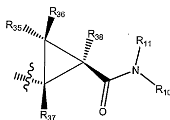
" trans -cyclopropanamide"
