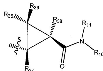
" trans -cyclopropanamide"
