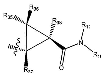
"trans-cyclopropanamide"
