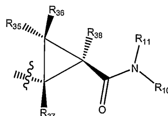
" trans -cyclopropanamide"
