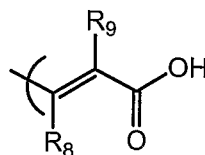
" trans -cinnamic acid"
