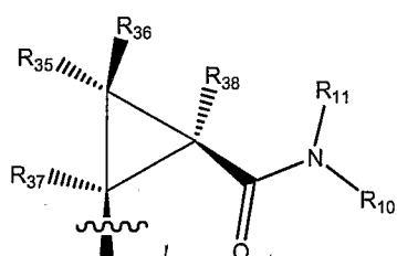
" cis -cyclopropanamide"
