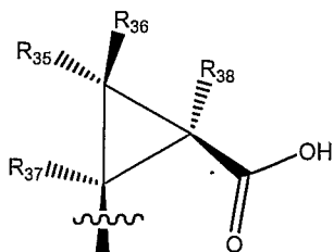
"cis-cyclopropanoic acid"
