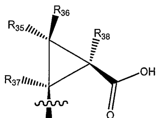
" cis -cyclopropanoic acid"
