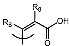
"cis-cinnamic acid"
