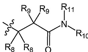
Formula VI
