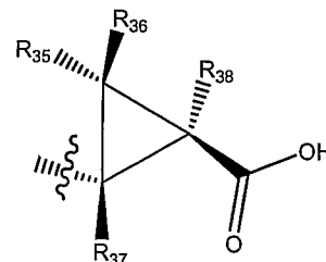
"trans-cyclopropanoic acid"
