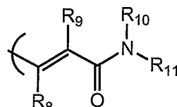
" trans -cinnamide"
