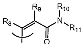
" cis -cinnamide"
