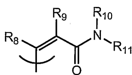
" cis -cinnamide"
