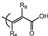
"trans-cinnamic acid"
