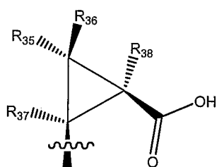
" cis -cyclopropanoic acid"
