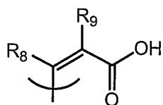
"cis-cinnamic acid"
