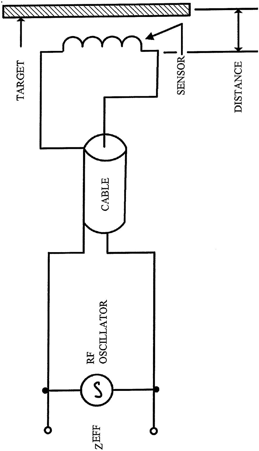
FIG. 1 (PRIOR ART)
