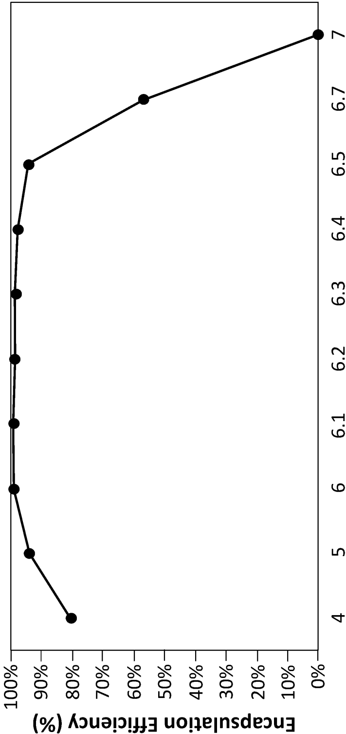
Buffer pH FIG. 25
