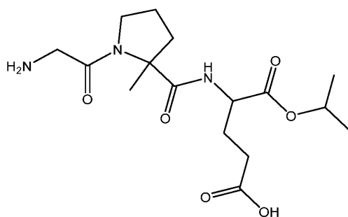
(VII) (Gly-MePro-Glu-OiPr),
