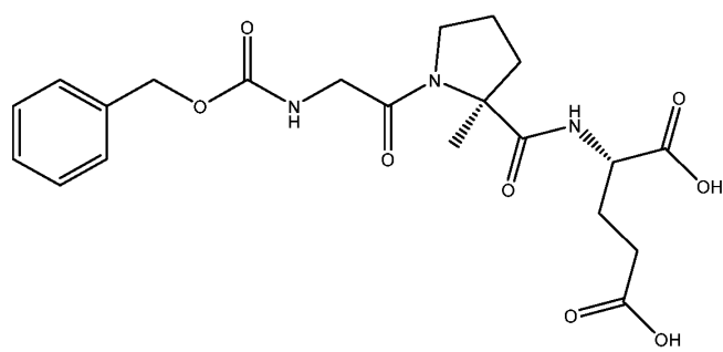
(IIa) Z-Gly-MePro-Glu-
