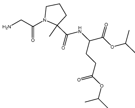
(VIII) (Gly-MePro-Glu-(OiPr) 2 ),
