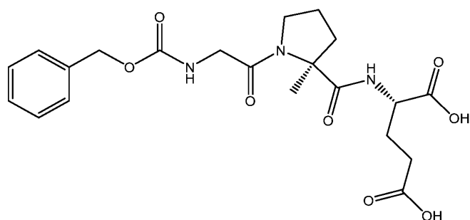
(IIa)(Z-Gly-MePro-Glu-
